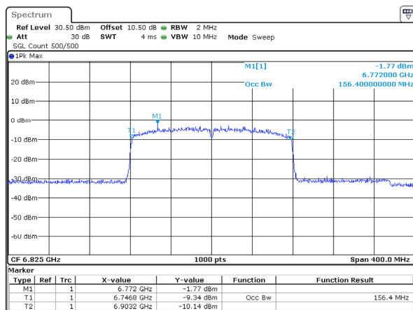
802.11ax160_6825MHz_RU_Full_Chain 3 156.400MHz
