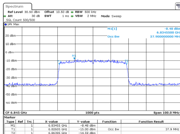
802.11ax40_6845MHz_RU_Full_Chain 1 37.900MHz
