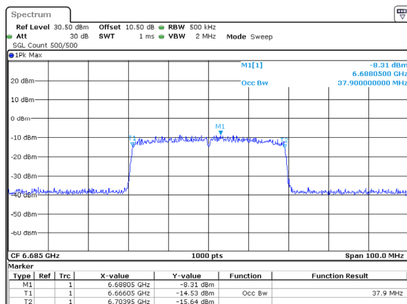
802.11ax40_6685MHz_RU_Full_Chain 1 37.900MHz
