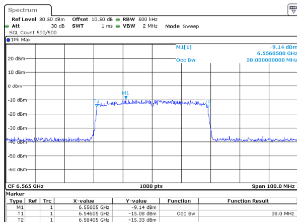
802.11ax40_6565MHz_RU_Full_Chain 0 38MHz
