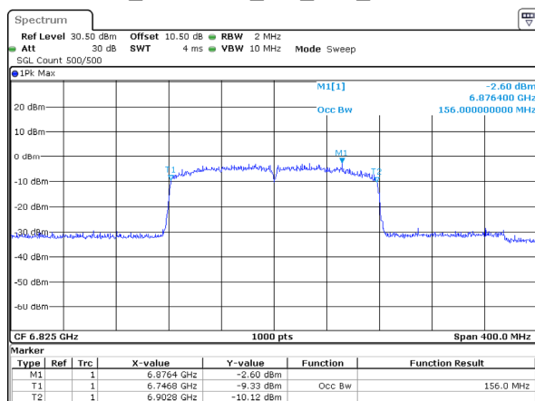
802.11ax160_6825MHz_RU_Full_Chain 1 156MHz
