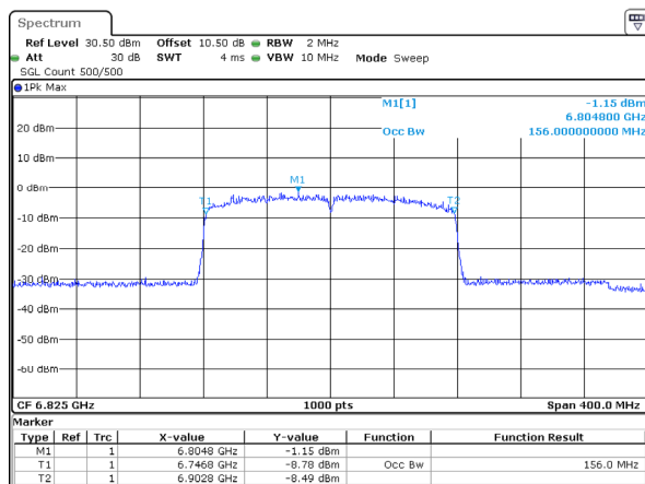
802.11ax160_6825MHz_RU_Full_Chain 2 156MHz
