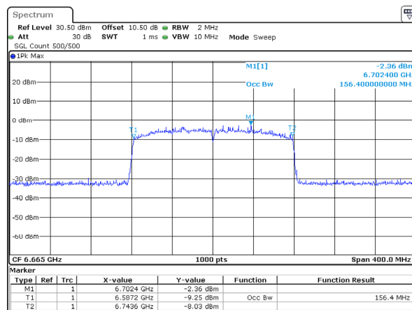
802.11ax160_6665MHz_RU_Full_Chain 3 156.400MHz
