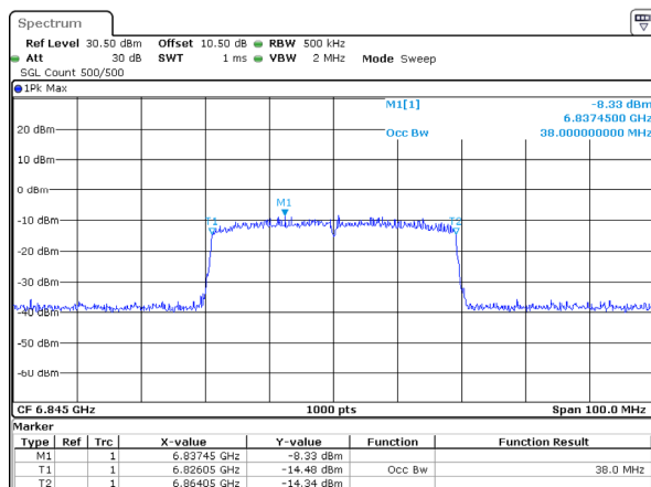
802.11ax40_6845MHz_RU_Full_Chain 0 38MHz
