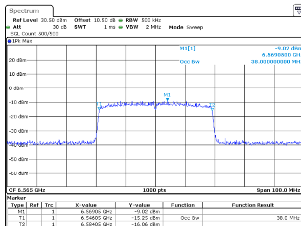
802.11ax40_6565MHz_RU_Full_Chain 1 38MHz
