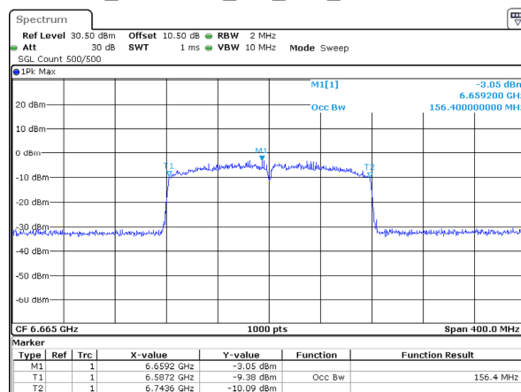
802.11ax160_6665MHz_RU_Full_Chain 1 156.400MHz
