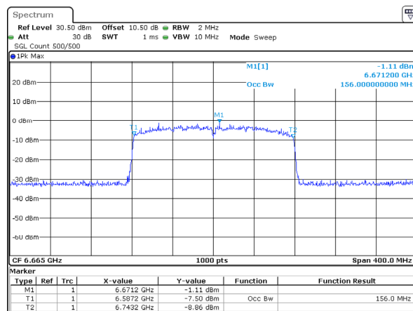
802.11ax160_6665MHz_RU_Full_Chain 2 156MHz
