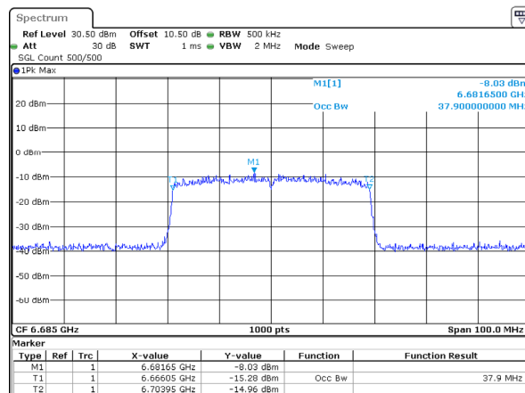
802.11ax40_6685MHz_RU_Full_Chain 0 37.900MHz
