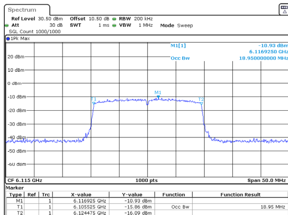
802.11ax20_6115MHz_RU_Full_Chain 2 18.950MHz
