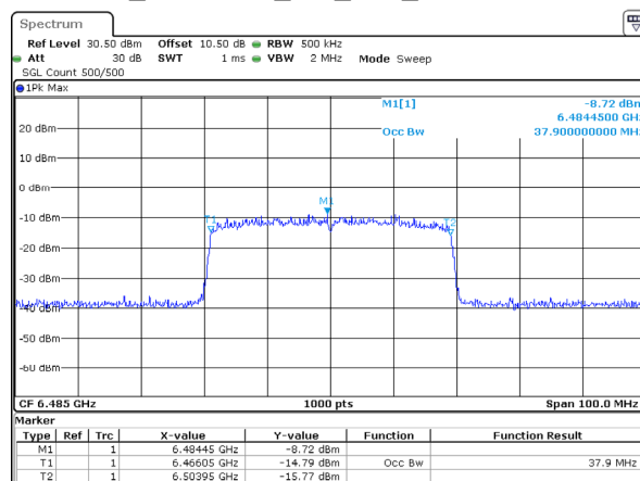
802.11ax40_6485MHz_RU_Full_Chain 1 37.900MHz
