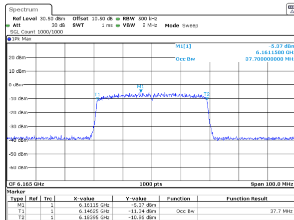
802.11ax40_6165MHz_RU_Full_Chain 0 37.700MHz
