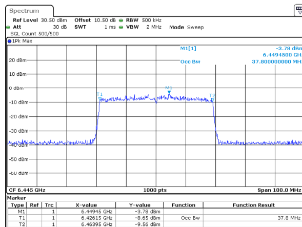
802.11ax40_6445MHz_RU_Full_Chain 2 37.800MHz
