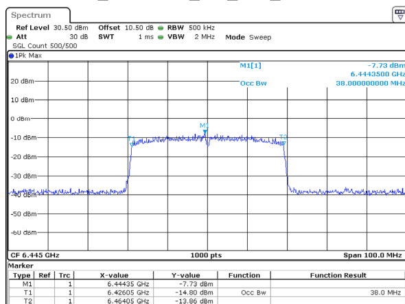
802.11ax40_6445MHz_RU_Full_Chain 1 38MHz
