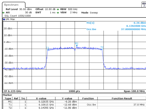
802.11ax40_6125MHz_RU_Full_Chain 0 37.800MHz
