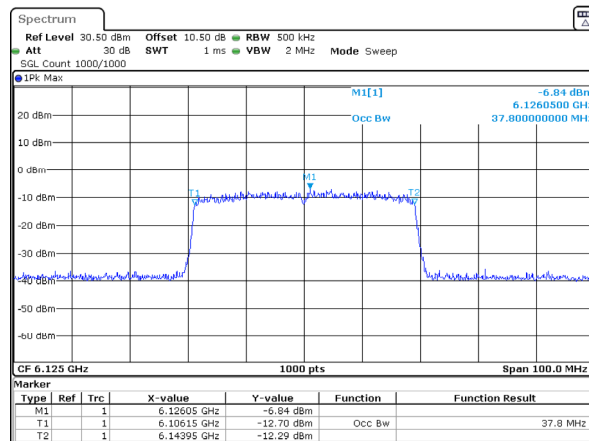
802.11ax40_6125MHz_RU_Full_Chain 1 37.800MHz
