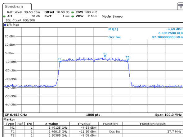
802.11ax40_6485MHz_RU_Full_Chain 2 37.700MHz
