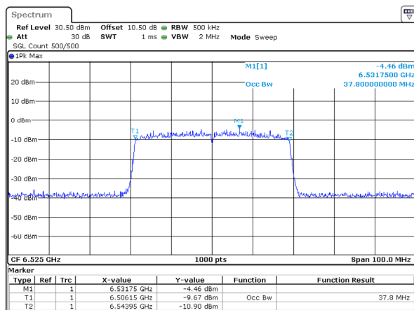
802.11ax40_6525MHz_RU_Full_Chain 2 37.800MHz
