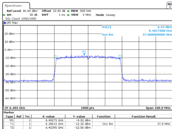
802.11ax40_6405MHz_RU_Full_Chain 0 37.800MHz
