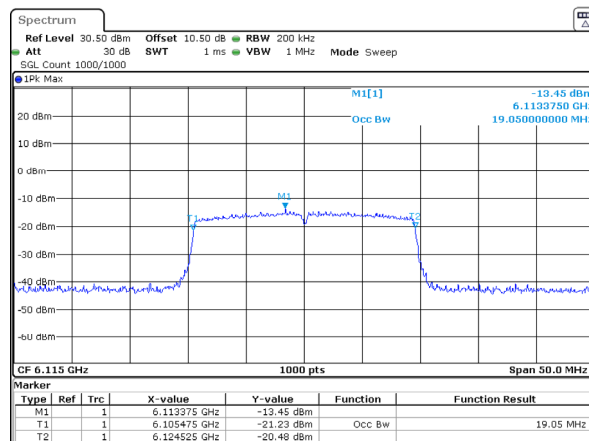
802.11ax20_6115MHz_RU_Full_Chain 3 19.050MHz
