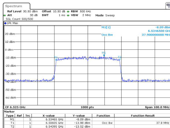
802.11ax40_6525MHz_RU_Full_Chain 3 37.900MHz
