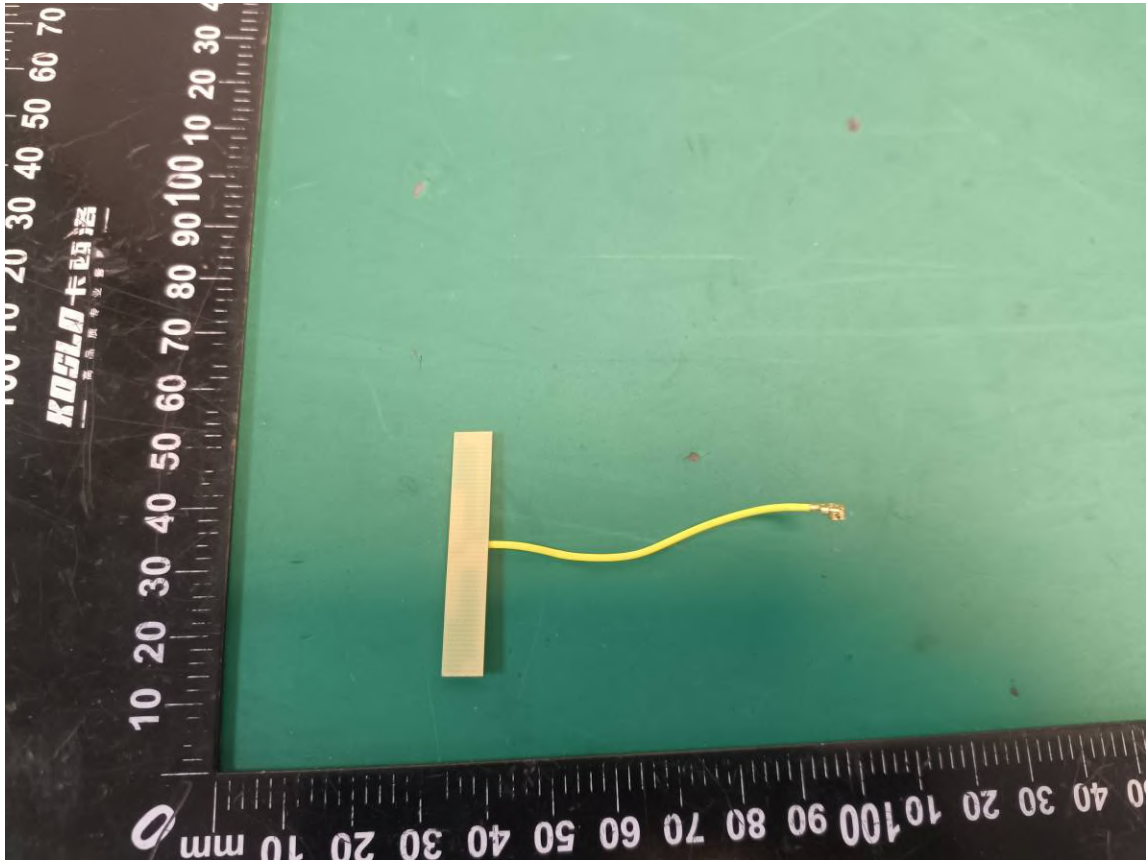
2.4G/5G Wi-Fi ANT2
