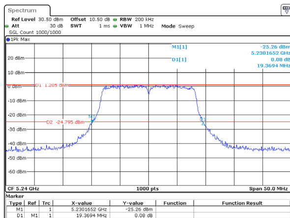
802.11a_5240MHz_Chain 2
