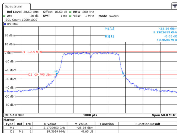
802.11a_5180MHz_Chain 3
