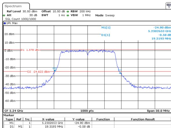
802.11a_5240MHz_Chain 3
