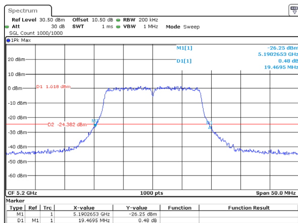
802.11a_5200MHz_Chain 3
