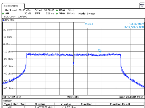
802.11ax20_2462MHz_RU_Full_Chain 3
