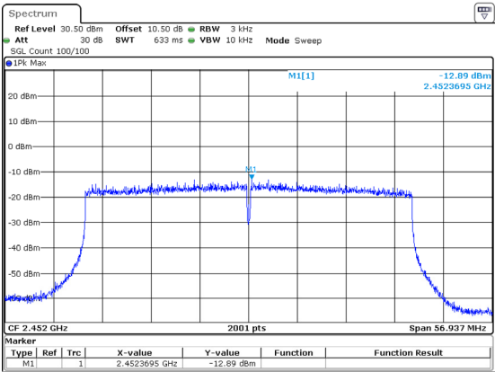
802.11ax40_2452MHz_RU_Full_Chain 2
