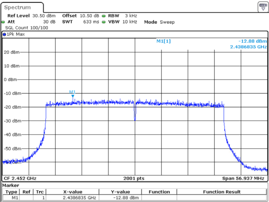
802.11ax40_2452MHz_RU_Full_Chain 3
