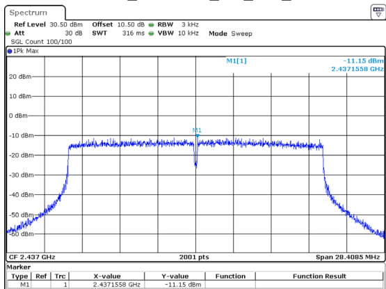
802.11ax20_2437MHz_RU_Full_Chain 2
