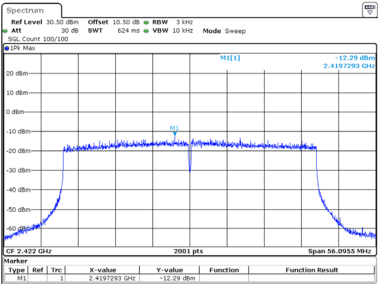
802.11ax40_2422MHz_RU_Full_Chain 2
