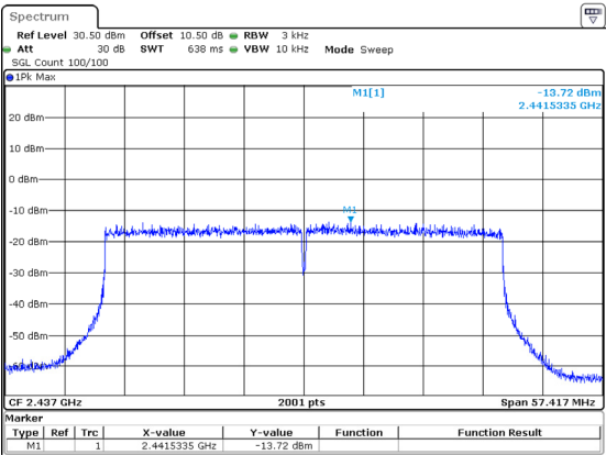
802.11ax40_2437MHz_RU_Full_Chain 2
