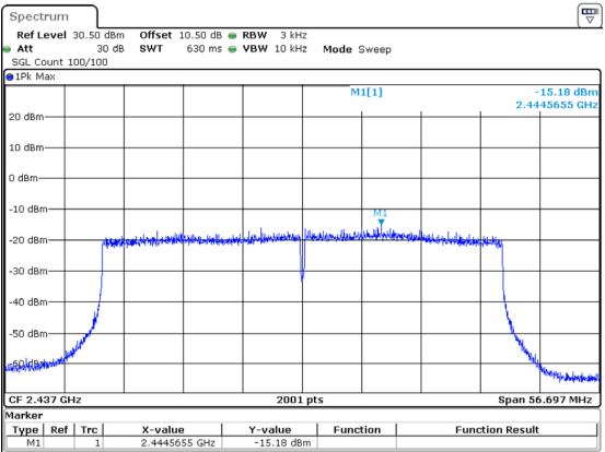
802.11ax40_2437MHz_RU_Full_Chain 0
