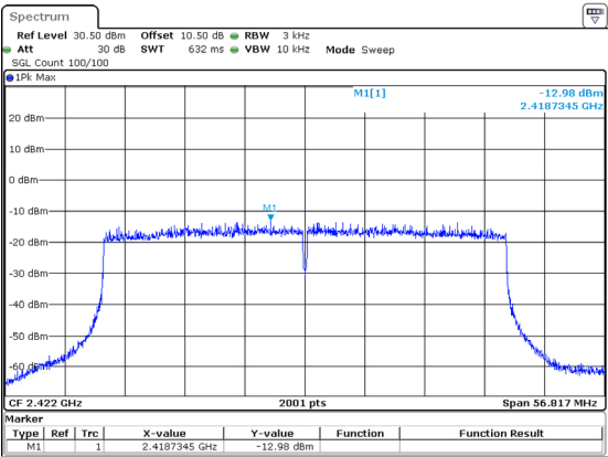
802.11ax40_2422MHz_RU_Full_Chain 3
