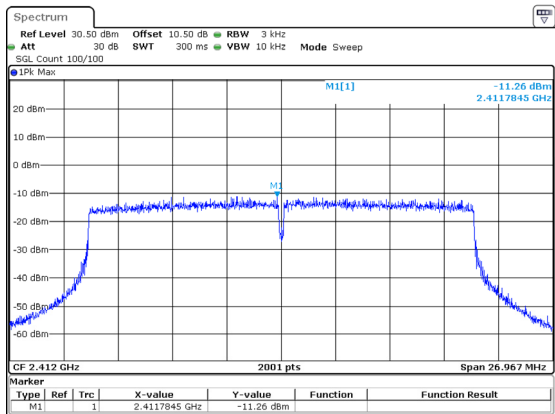
802.11ax20_2412MHz_RU_Full_Chain 3
