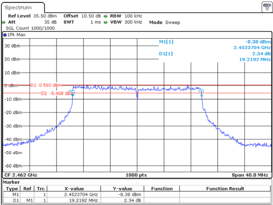
802.11ax20_2462MHz_RU_Full_Chain 0
