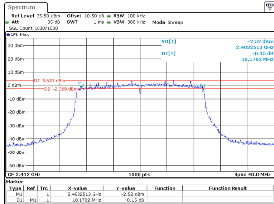
802.11ax20_2412MHz_RU_Full_Chain 2
