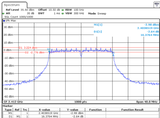
802.11g_2412MHz_Chain 3
