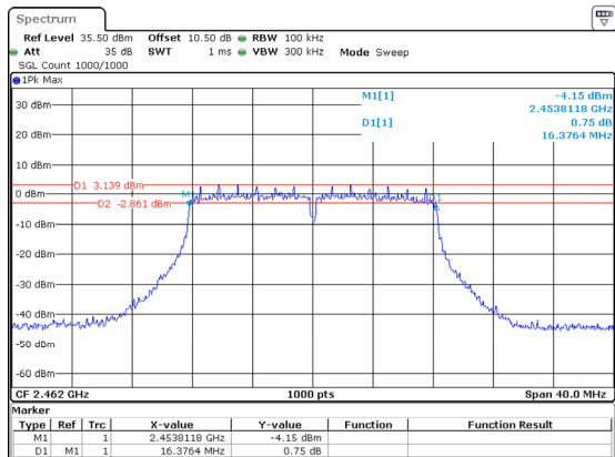
802.11g_2462MHz_Chain 2
