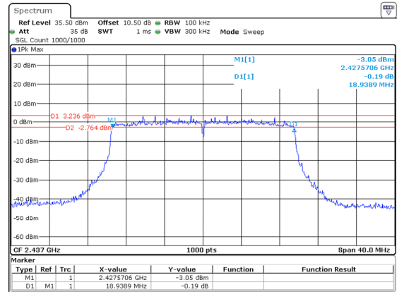
802.11ax20_2437MHz_RU_Full_Chain 2
