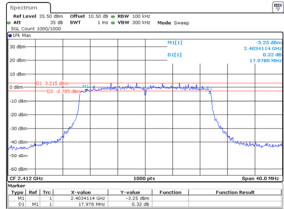
802.11ax20_2412MHz_RU_Full_Chain 3
