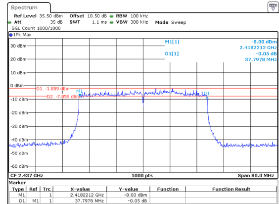
802.11ax40_2437MHz_RU_Full_Chain 0
