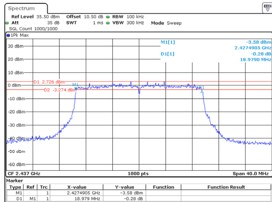
802.11ax20_2437MHz_RU_Full_Chain 3
