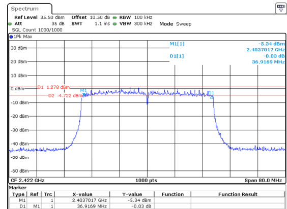
802.11ax40_2422MHz_RU_Full_Chain 1
