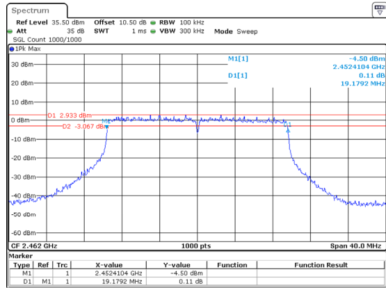
802.11ax20_2462MHz_RU_Full_Chain 2
