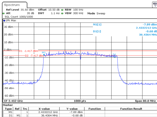
802.11ax40_2452MHz_RU_Full_Chain 0
