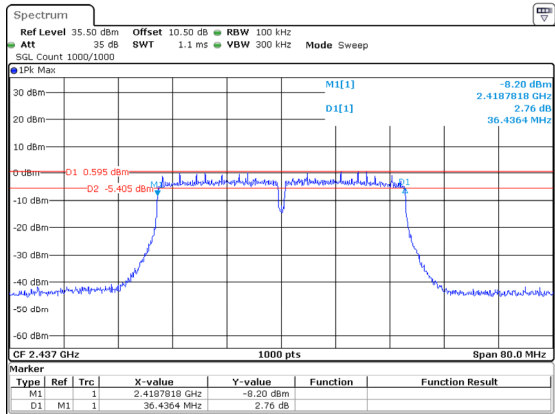
802.11n40_2437MHz_Chain 2
