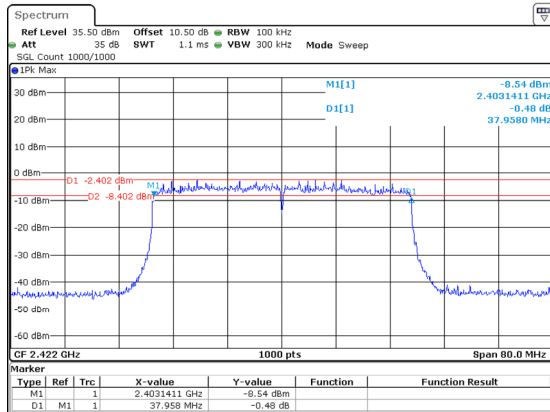
802.11ax40_2422MHz_RU_Full_Chain 0
