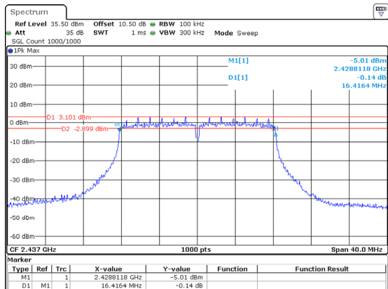
802.11g_2437MHz_Chain 3
