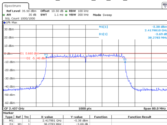
802.11ax40_2437MHz_RU_Full_Chain 1
