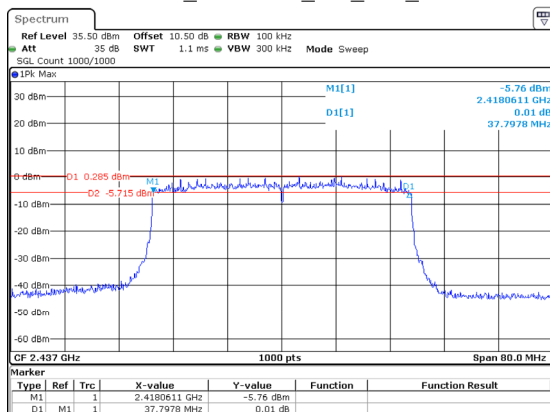
802.11ax40_2437MHz_RU_Full_Chain 3
