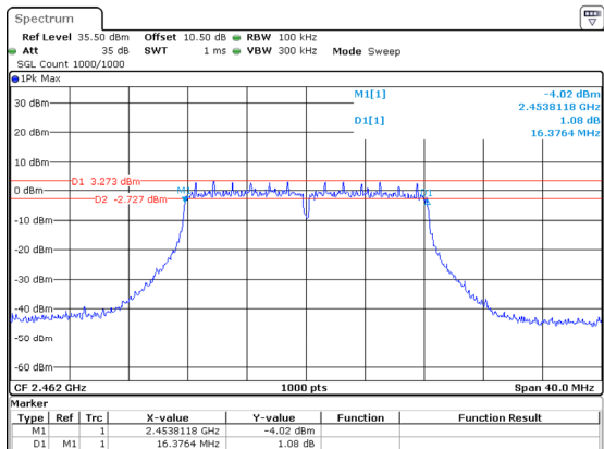
802.11g_2462MHz_Chain 3
