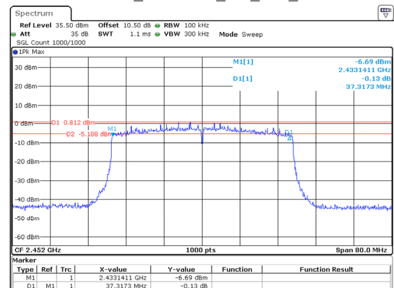
802.11ax40_2452MHz_RU_Full_Chain 1
