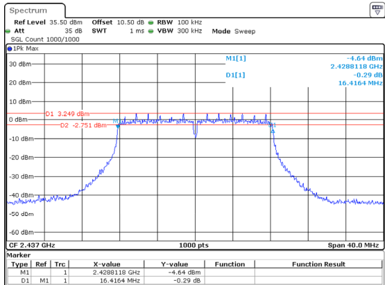
802.11g_2437MHz_Chain 2
