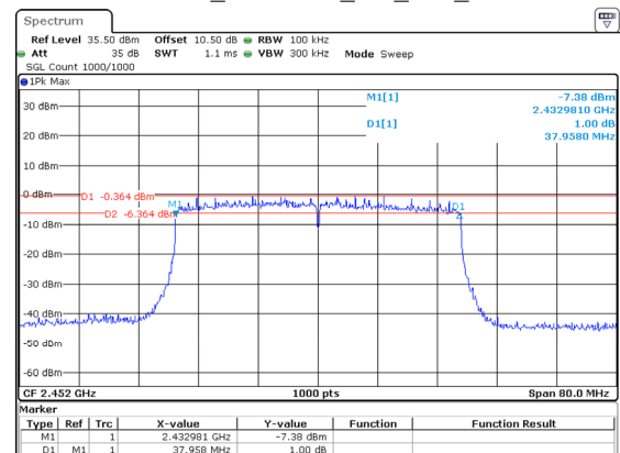
802.11ax40_2452MHz_RU_Full_Chain 3
