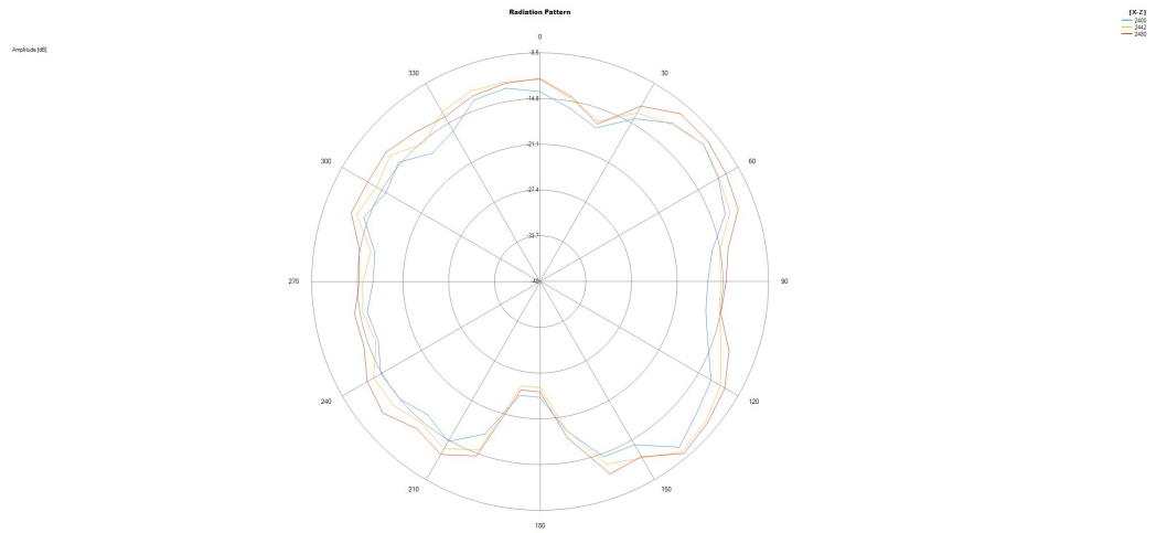
Y-Z Plane
