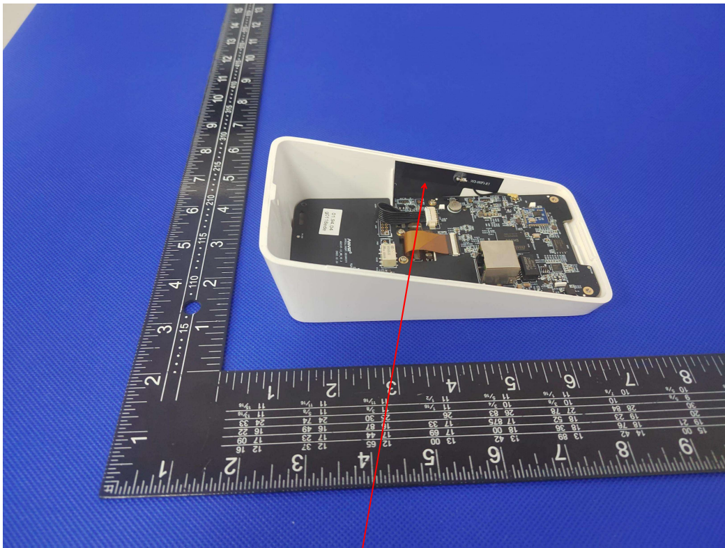
WIFI ANT
