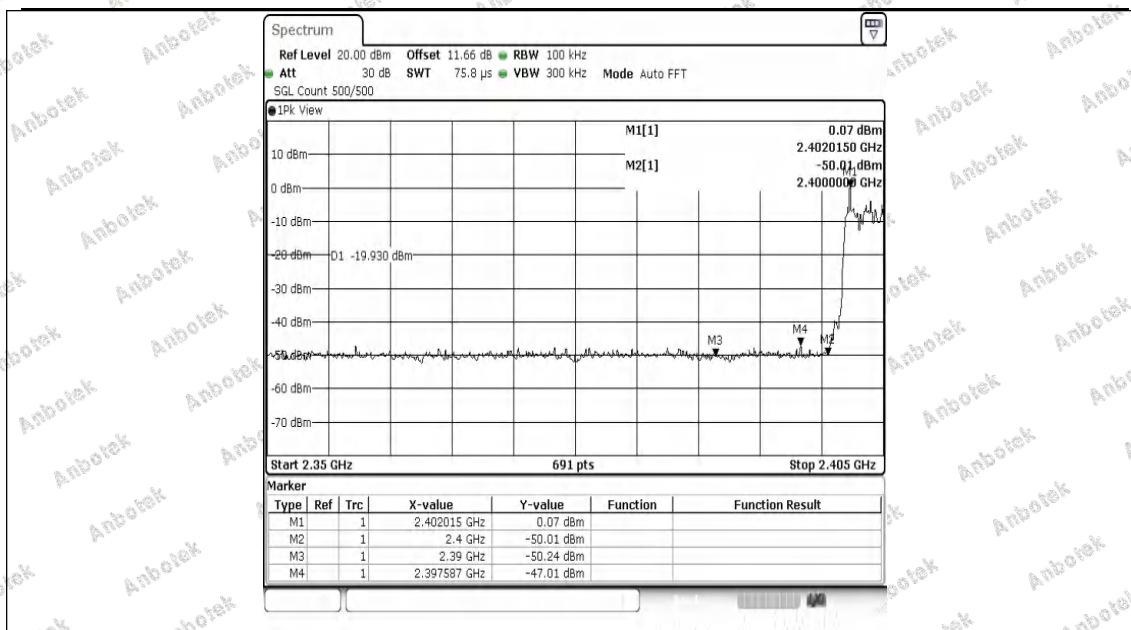
3DH5-Ant1-Hop_2402-PASS
