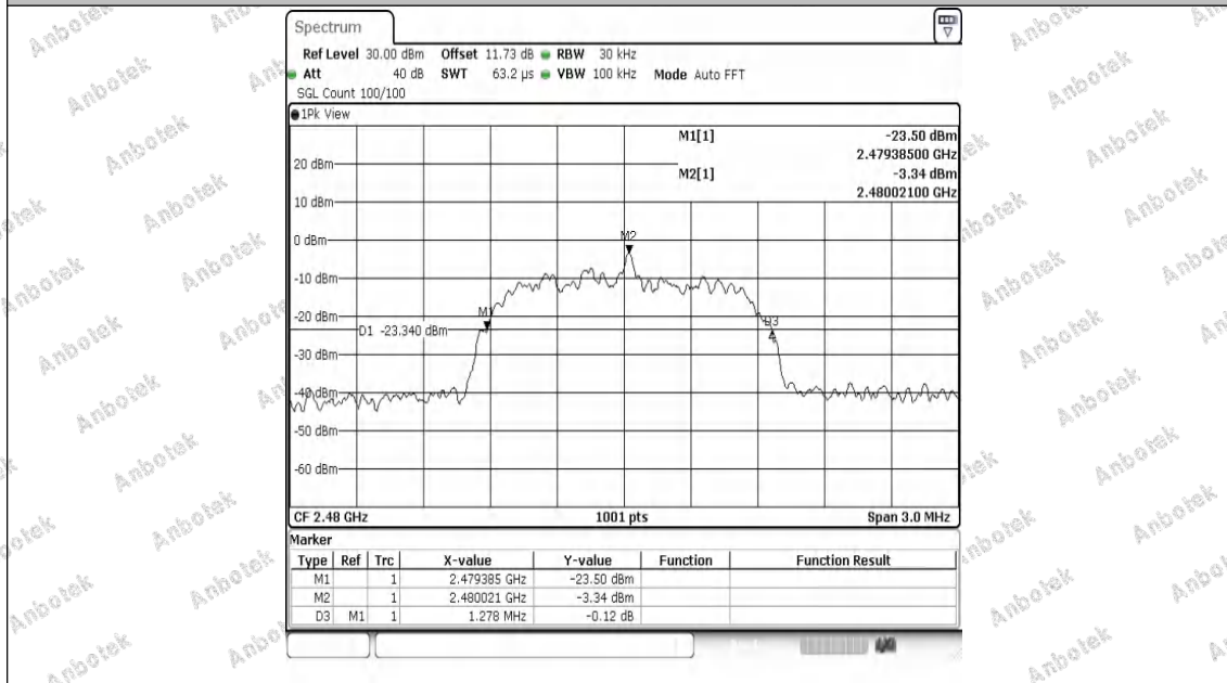
2DH5-Ant1-2480
