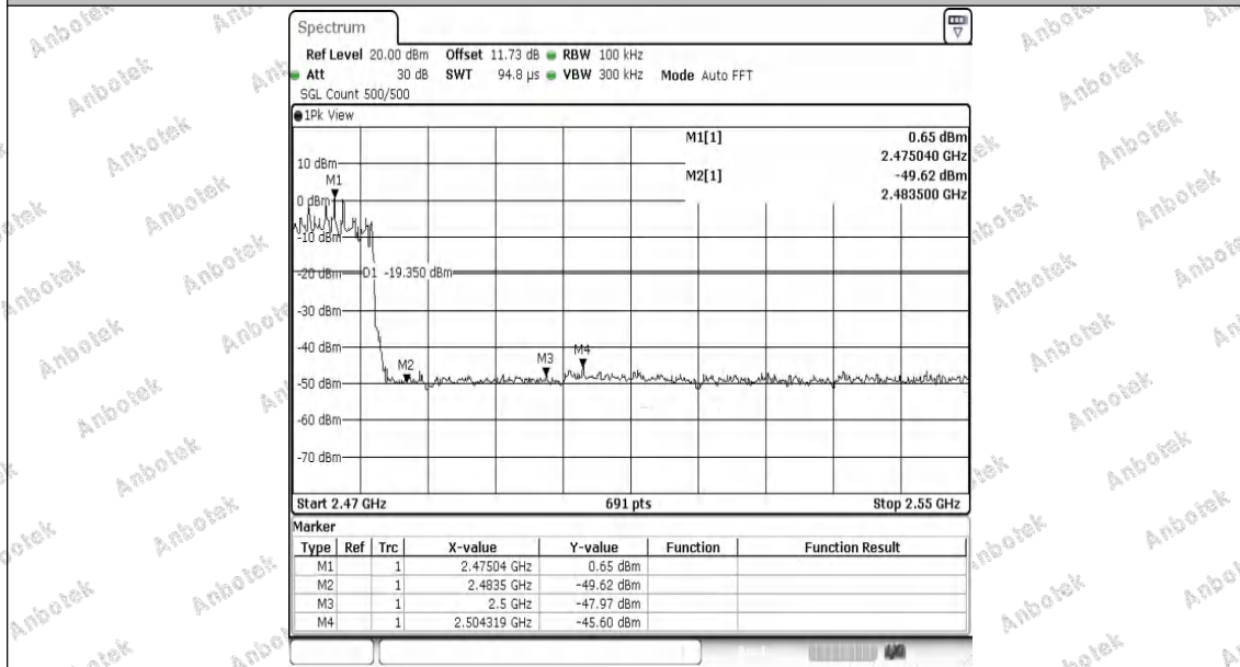
3DH5-Ant1-Hop_2480-PASS
