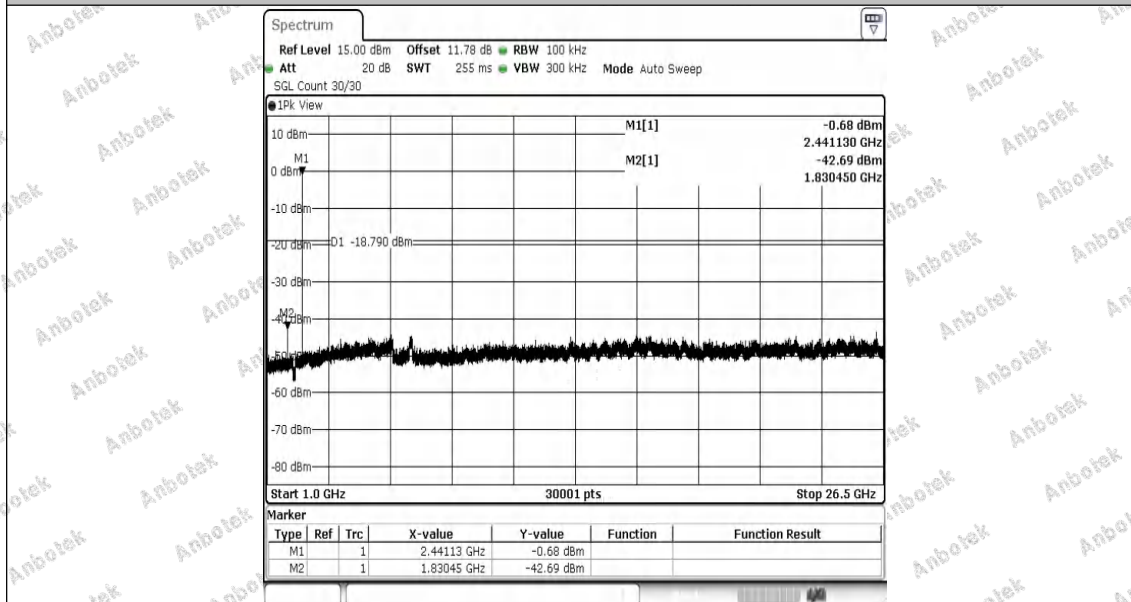
3DH5-Ant1-2441-1000~26500-PASS
