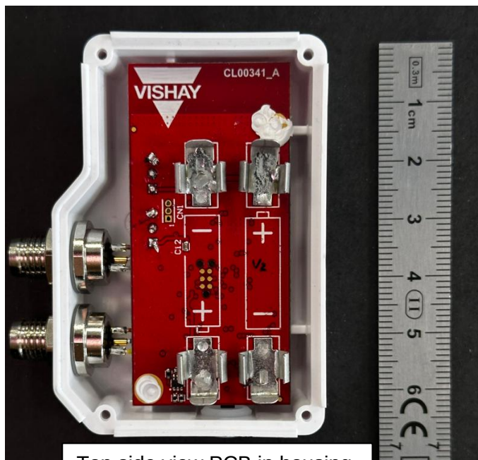
Top side view PCB in housing
