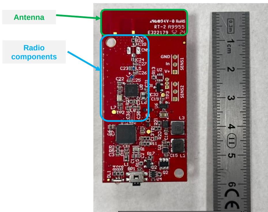
Bottom side view PCB alone
