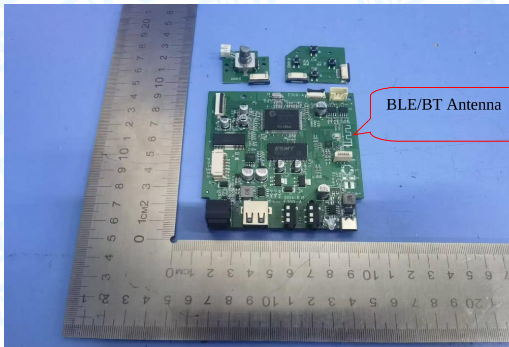
Photo 9 Appearance of PCB
