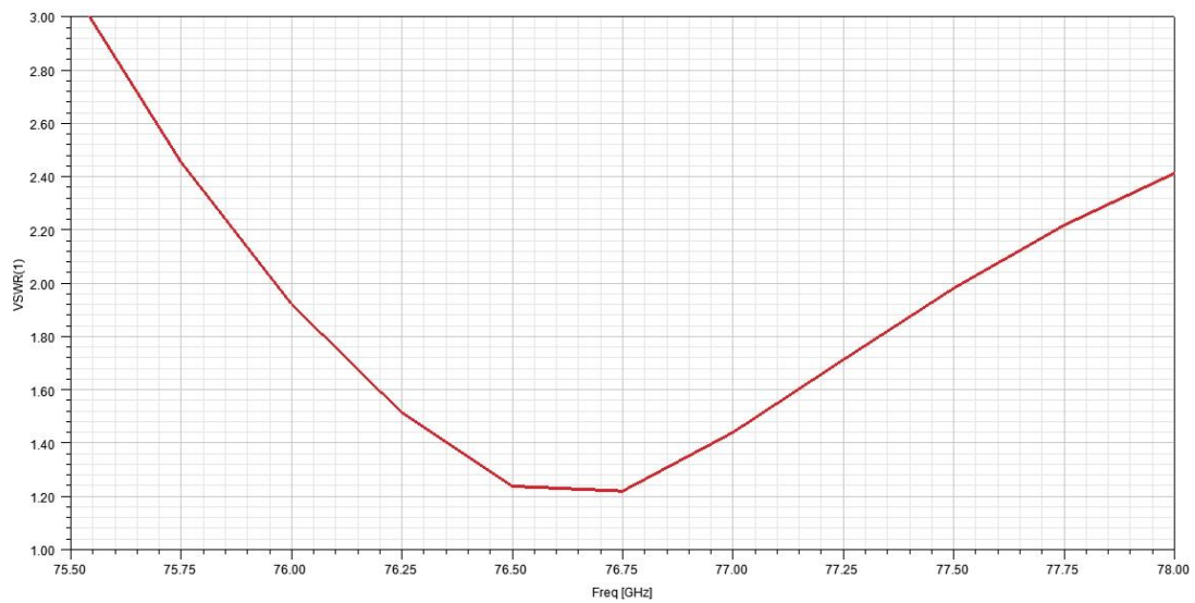
Voltage Standing Wave Ratio (VSWR)
