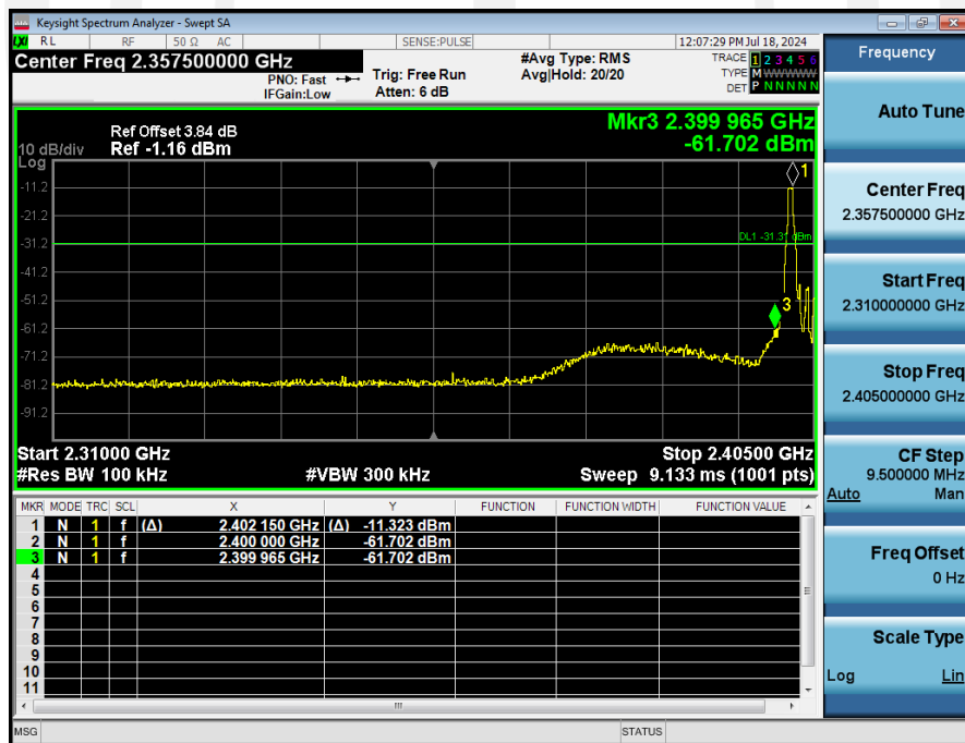
2_Bandedge_NVNT_ANT1_1-DH1_2402
