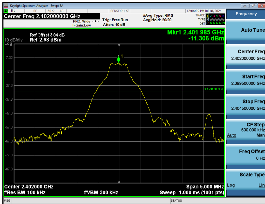
2_Bandedge_NVNT_ANT1_1-DH1_2402
