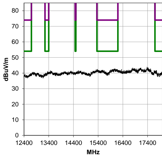
12400-18000 MHz, Run 229
