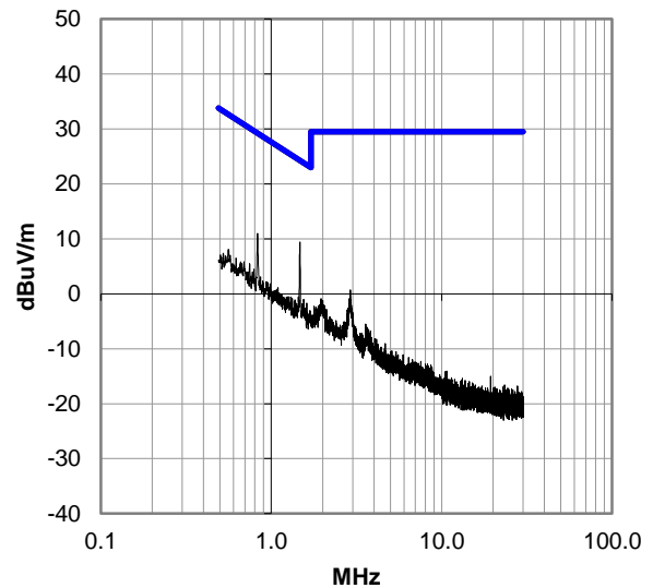
0.49-30 MHz, Run 235
