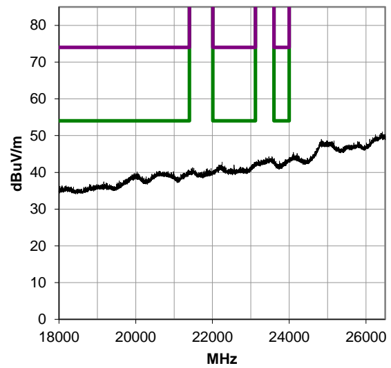
18000-26500 MHz, Run 231
