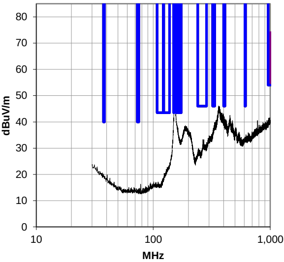
30-1000 MHz, Run 75 Emission near the limit does not fall in a restricted band.
