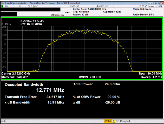
20 MHz BW Low Channel 5, 2432 MHz 802.11(b) 1 Mbps
