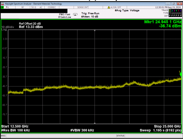
20 MHz BW Mid Channel 7, 2442 MHz 802.11(b) 1 Mbps
