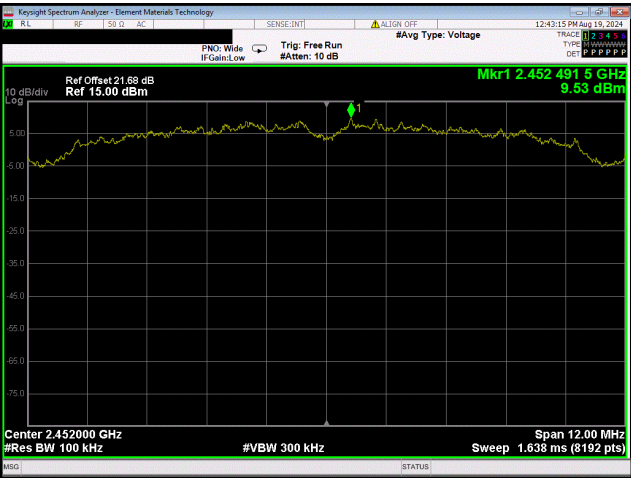
20 MHz BW High Channel 9, 2452 MHz 802.11(b) 1 Mbps
