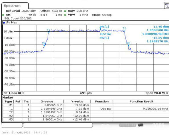
Band25 QAM16 BW=10MHz Channel=26090 RB Size=50 Position=#0
