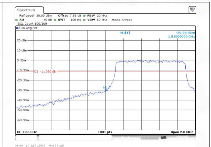
Band25 QAM16 BW=1.4MHz Channel=26047 RB Size=6 Position=#0
