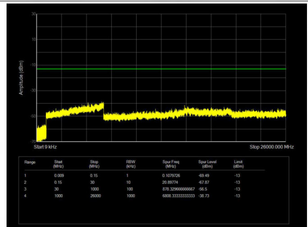
Band25 QAM16 BW=15MHz Channel=26115 RB Size=75 Position=#0
