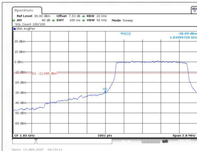
Band25 QPSK BW=1.4MHz Channel=26047 RB Size=6 Position=#0
