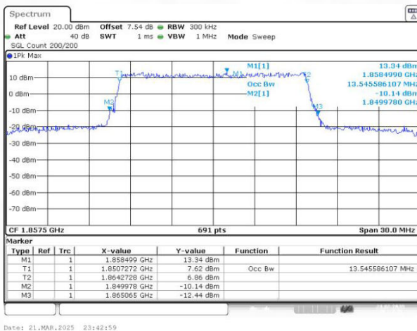
Band25 QAM16 BW=15MHz Channel=26115 RB Size=75 Position=#0
