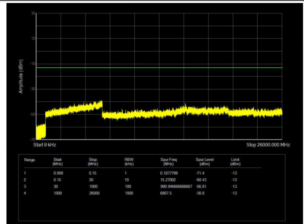
Band25 QAM16 BW=10MHz Channel=26640 RB Size=50 Position=#0
