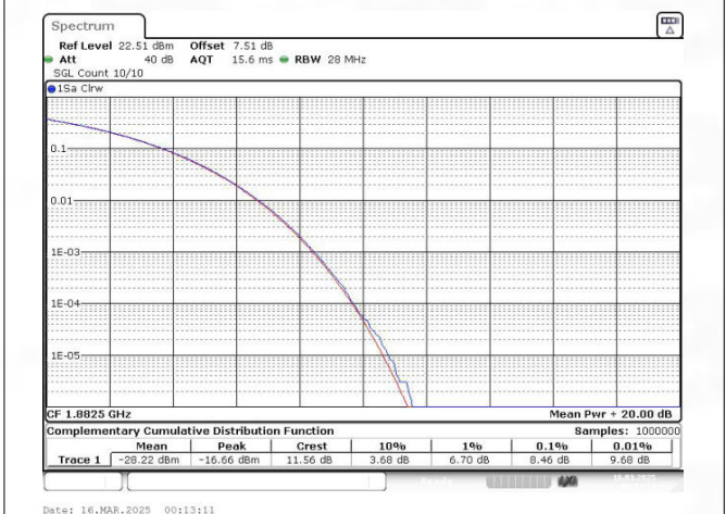
Band25 QAM16 BW=3MHz Channel=26365 RB Size=1 Position=#0
