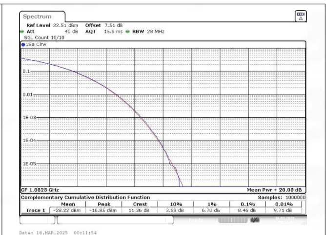
Band25 QAM16 BW=1.4MHz Channel=26365 RB Size=1 Position=#0
