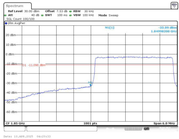
Band25 QAM16 BW=3MHz Channel=26055 RB Size=15 Position=#0
