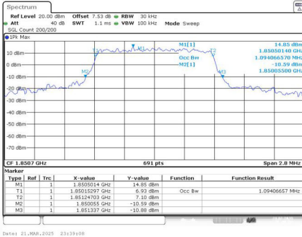
Band25 QAM16 BW=1.4MHz Channel=26047 RB Size=6 Position=#0
