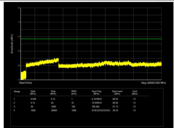
Band25 QAM16 BW=5MHz Channel=26665 RB Size=25 Position=#0
