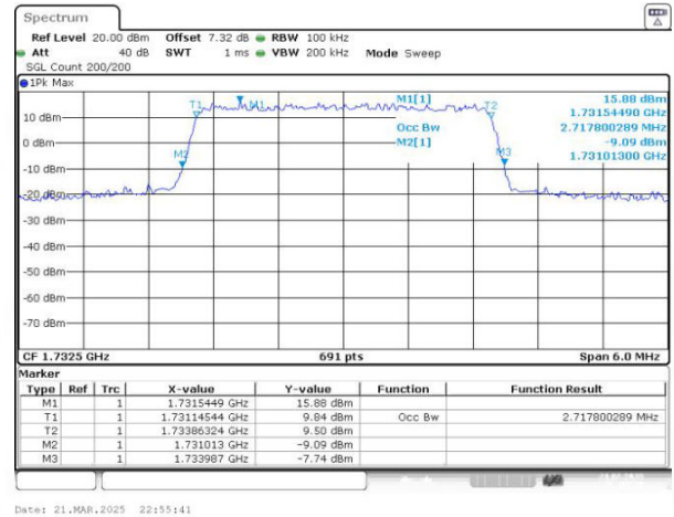
Band4 QAM16 BW=3MHz Channel=20175 RB Size=15 Position=#0
