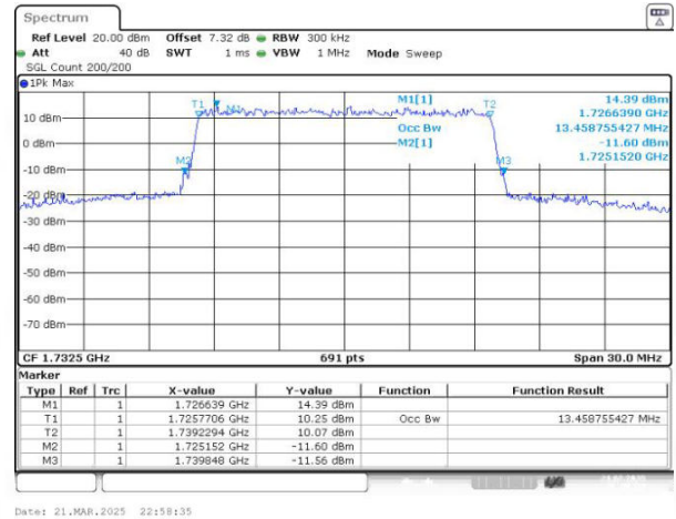
Band4 QAM16 BW=15MHz Channel=20175 RB Size=75 Position=#0
