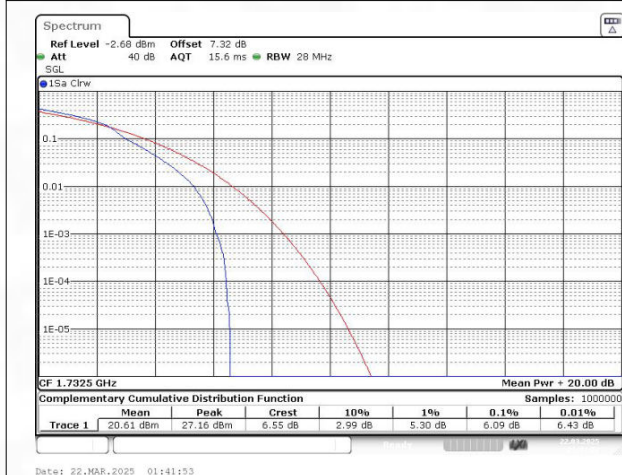
Band4 QAM16 BW=15MHz Channel=20175 RB Size=1 Position=#0
