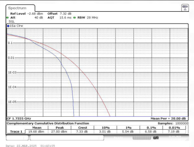
Band4 QAM16 BW=20MHz Channel=20175 RB Size=1 Position=#0
