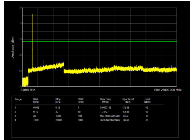
Band4 QPSK BW=3MHz Channel=20385 RB Size=15 Position=#0
