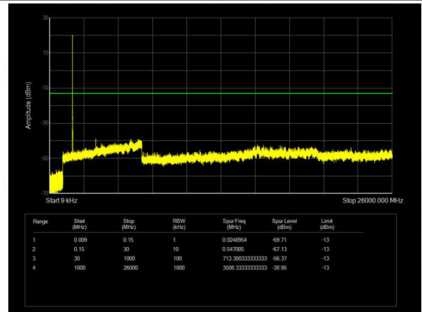
Band4 QPSK BW=5MHz Channel=20375 RB Size=25 Position=#0
