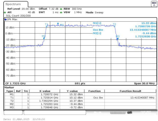
Band4 QPSK BW=15MHz Channel=20175 RB Size=75 Position=#0
