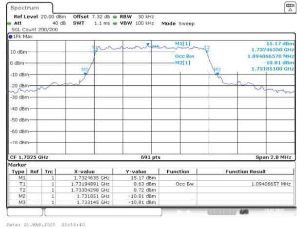
Band4 QPSK BW=1.4MHz Channel=20175 RB Size=6 Position=#0
