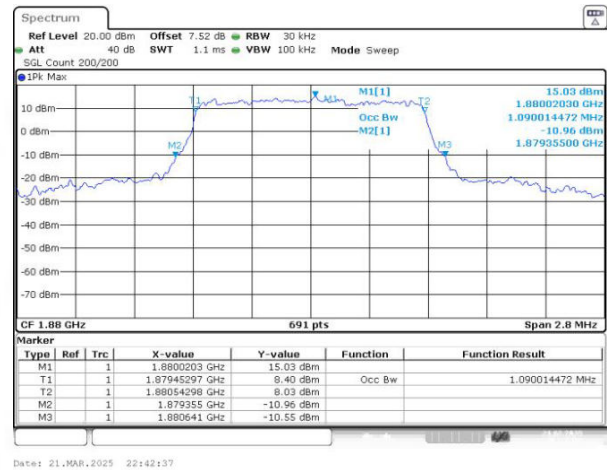
Band2 QAM16 BW=1.4MHz Channel=18900 RB Size=6 Position=#0
