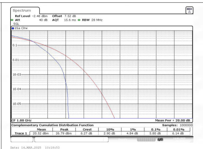
Band2 QAM16 BW=1.4MHz Channel=18900 RB Size=1 Position=#0
