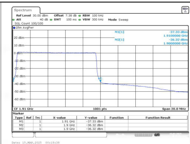
Band2 QAM16 BW=10MHz Channel=19150 RB Size=50 Position=#0
