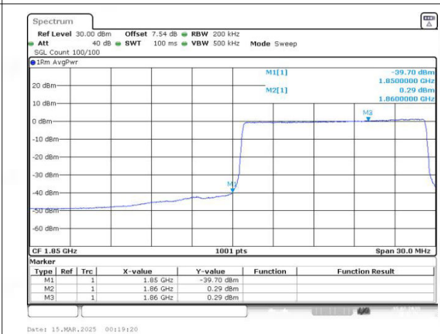
Band2 QAM16 BW=15MHz Channel=18675 RB Size=75 Position=#0
