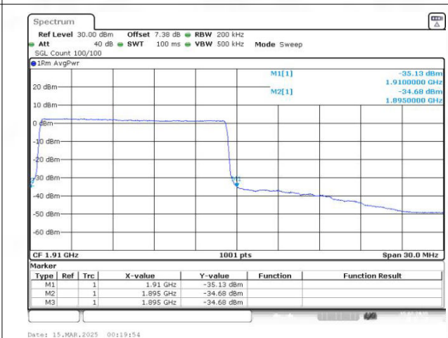
Band2 QAM16 BW=15MHz Channel=19125 RB Size=75 Position=#0
