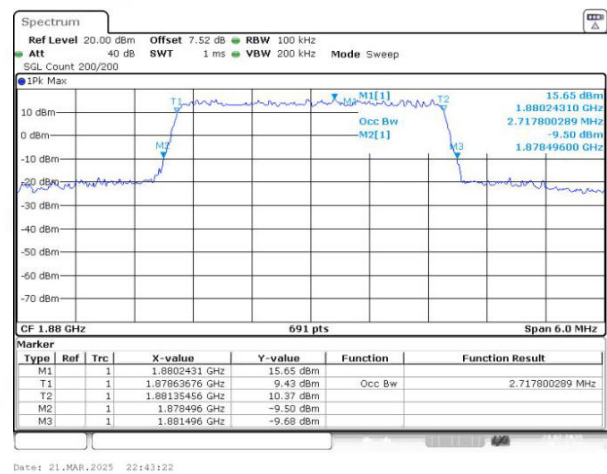
Band2 QAM16 BW=3MHz Channel=18900 RB Size=15 Position=#0
