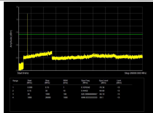
Band2 QAM16 BW=3MHz Channel=18615 RB Size=15 Position=#0
