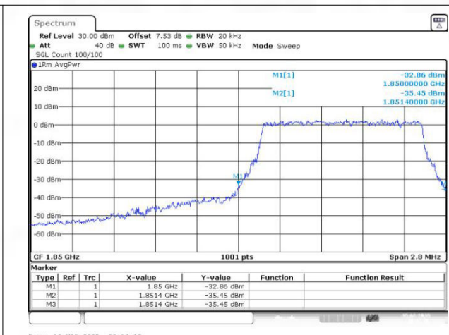
Band2 QAM16 BW=1.4MHz Channel=18607 RB Size=6 Position=#0
