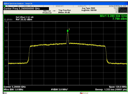
IEEE 802.11ac_Channel 58_80MHz_Antenna 0
