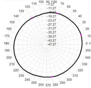
Total(H-XY), Max=-11.56dBi, CirD=6.17
