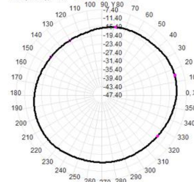
Total(H-XY), Max=-11.74dBi, CirD=5.90
