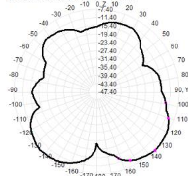
2430.0MHz Total(E2-YZ), Max=-7.51dBi
