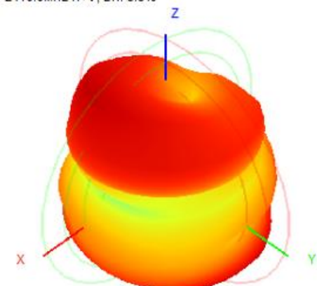
2410.0MHz H+V, Eff: 5.3%
