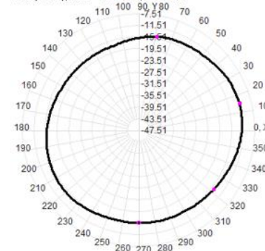
Total(H-XY), Max=-11.71dBi, CirD=5.76
