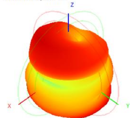
2400.0MHz H+V, Eff: 6.0%
