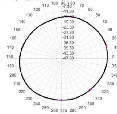
Total(H-XY), Max=-11.40dBi, CirD=6.01
