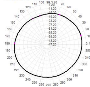
Total(H-XY), Max=-11.93dBi, CirD=6.34
