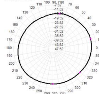
Total(H-XY), Max=-11.33dBi, CirD=5.81
