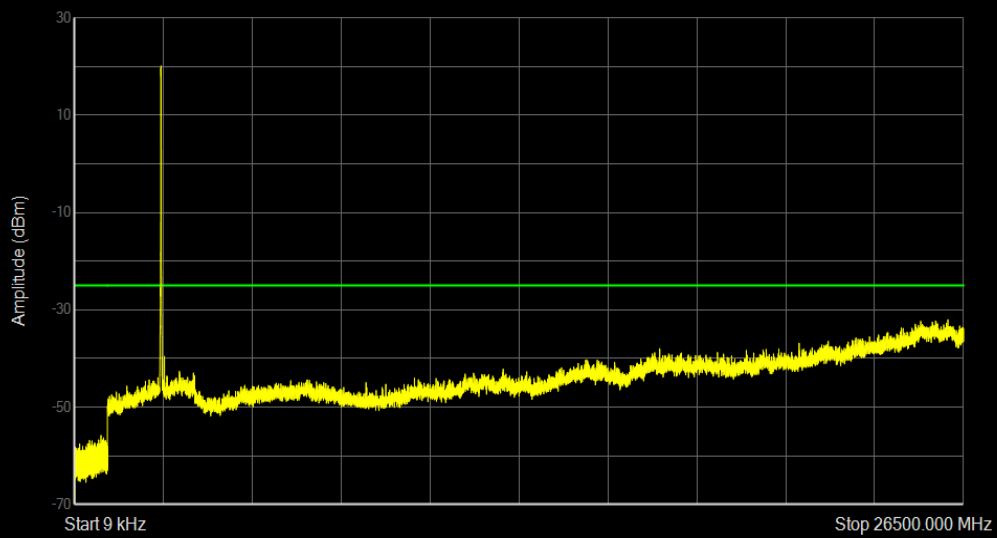
Band41(2535-2655) 16QAM BW=10MHz Channel=40640 RB Size=50 Position=#0
