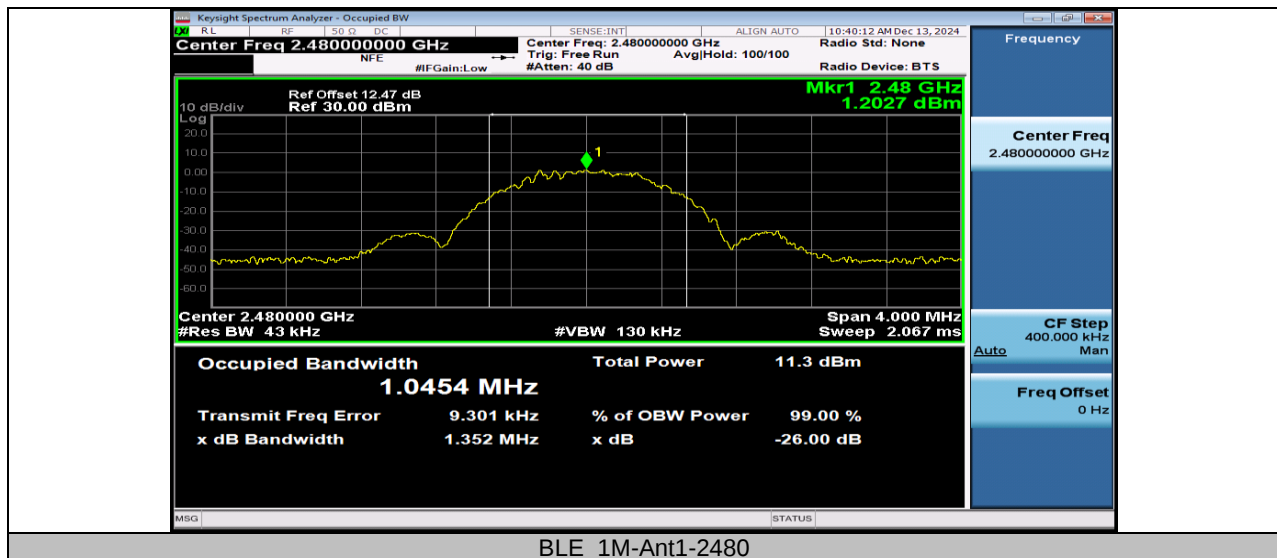
BLE_1M-Ant1-2480
