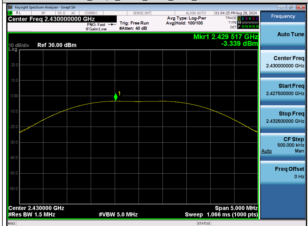
Test_Graph_GFSK_ANT1_2430_Peak Power
