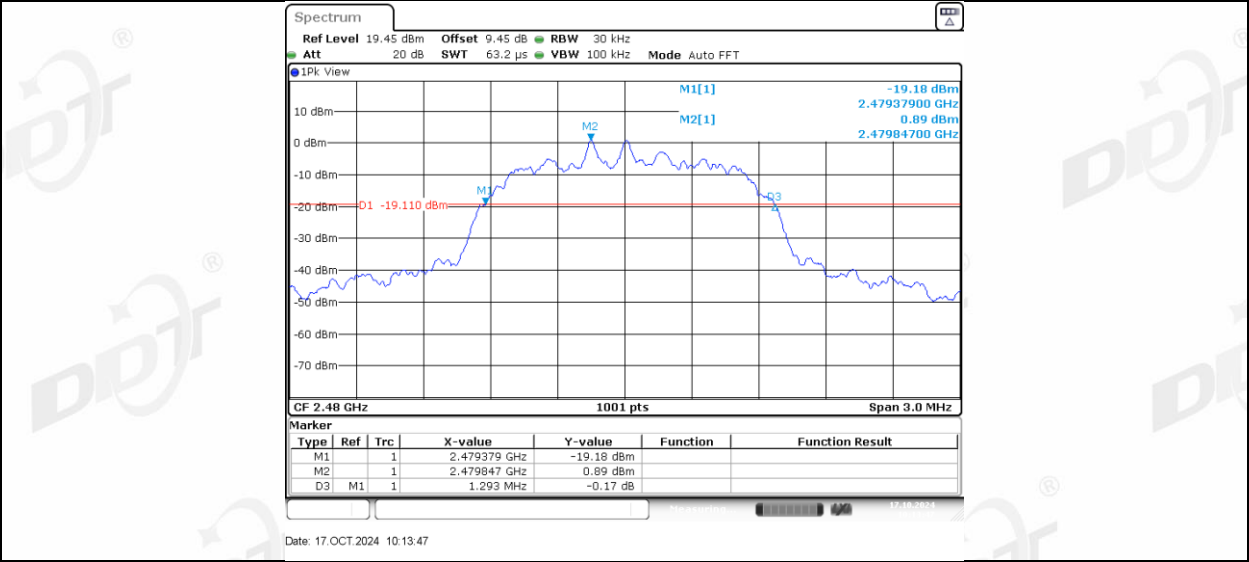
2DH5_Right side_2480
