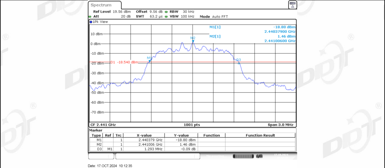
2DH5_Right side_2441
