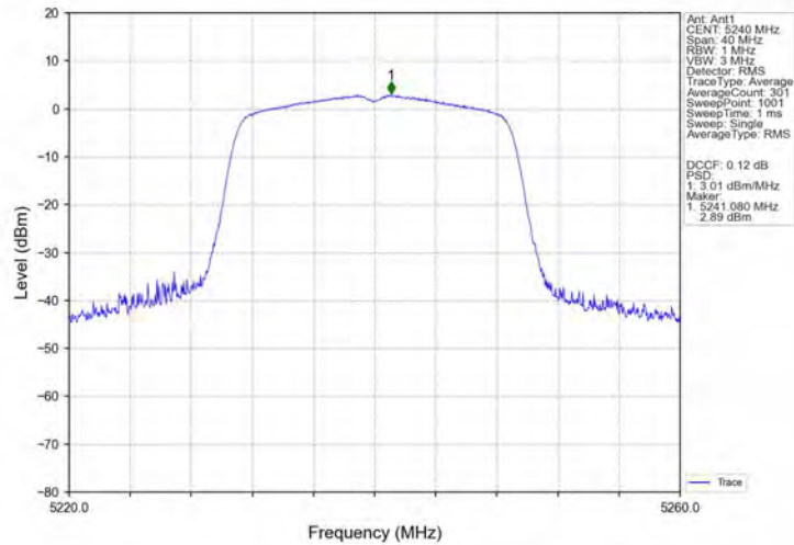
802.11n(HT20)_HCH_5240MHz_Ant1_NTNV
