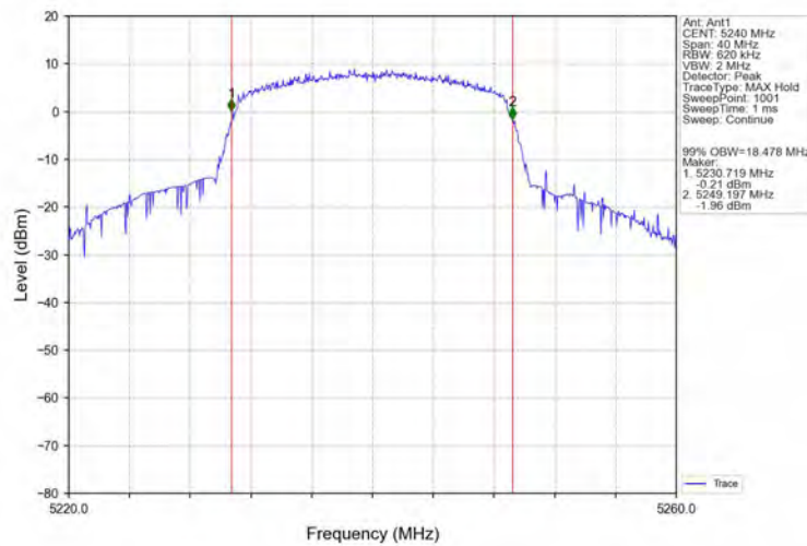
802.11n(HT20)_HCH_5240MHz_Ant1_NTNV
