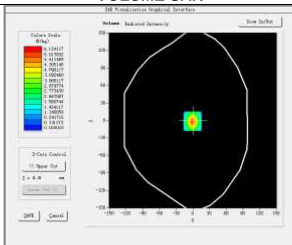
VOLUME SAR
