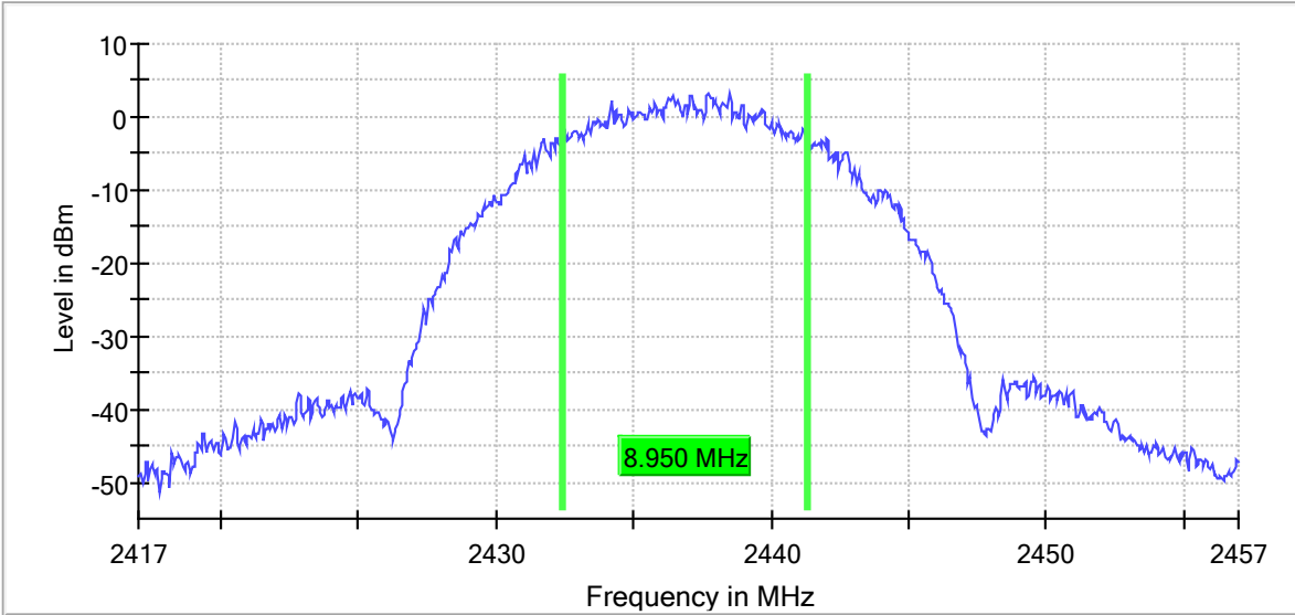
6 dB Bandwidth
