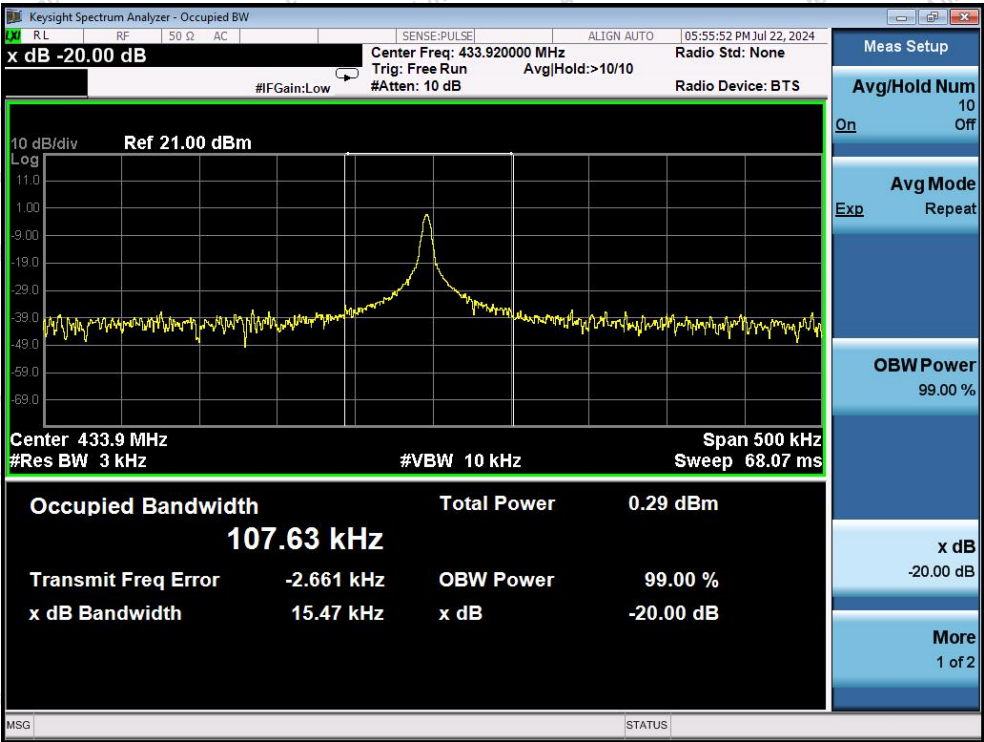
20dB Bandwidth
