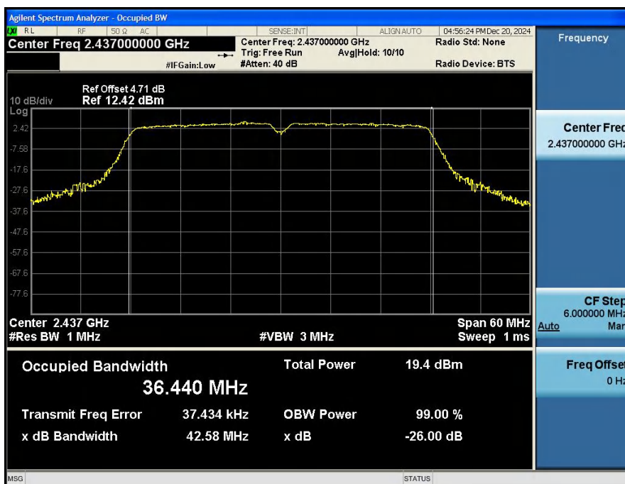
99%_Occupied_Bandwidth_NVNT_ANT1_802_11n(HT40)_2437
