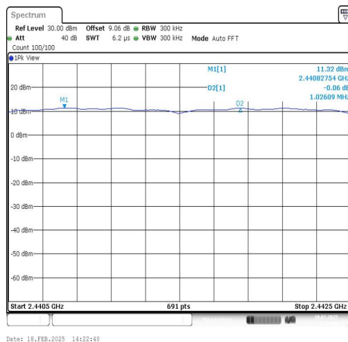
2DH5-Ant1-Hop-PASS
