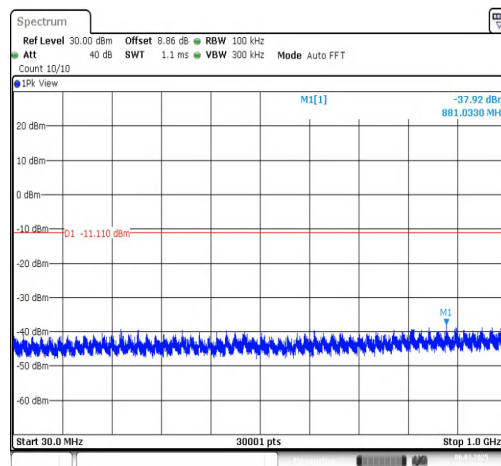
DH5-Ant1-2402-30~1000-PASS
