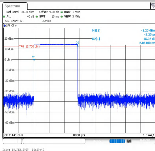
DH3-Ant1-Hop-PASS
