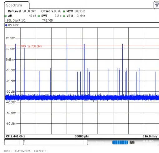
DH1-Ant1-Hop-PASS
