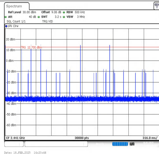
DH3-Ant1-Hop-PASS
