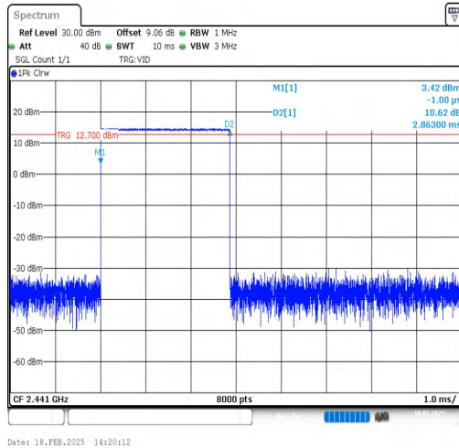
DH1-Ant1-Hop-PASS
