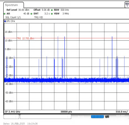
DH5-Ant1-Hop-PASS
