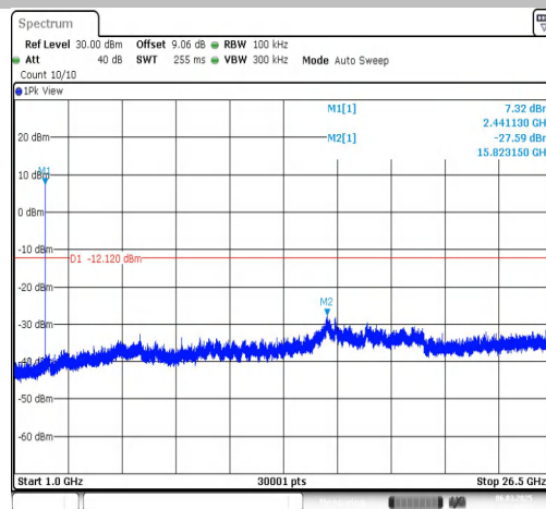
DH5-Ant1-2441-0~Reference-PASS
