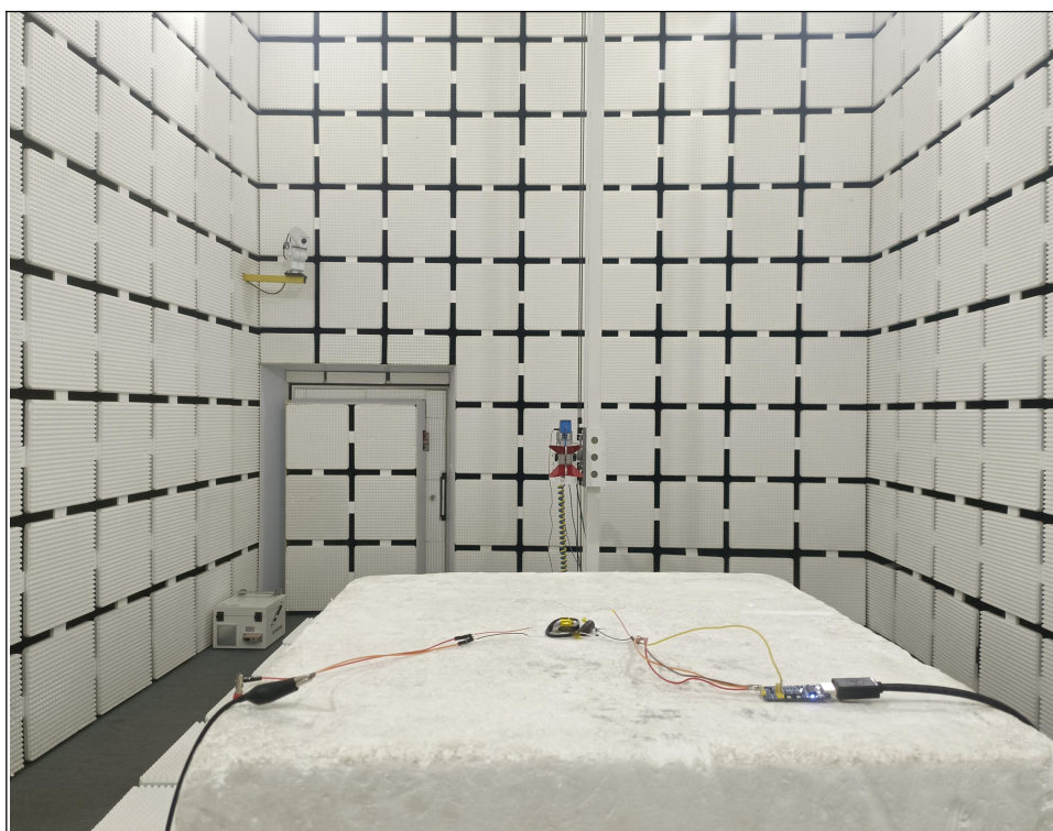
RADIATED EMISSION TEST (Above 1GHz)
