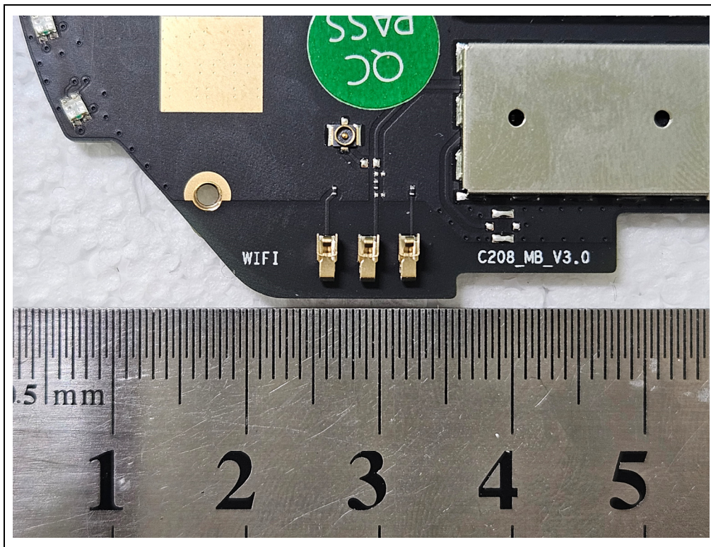
Ant Connector
