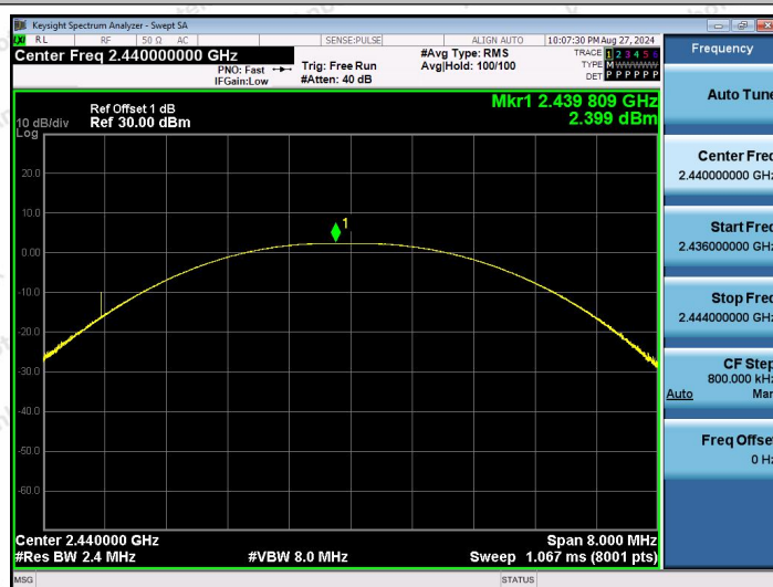
BLE_1M-Ant1-2440-PASS
