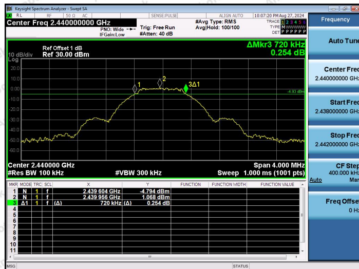
BLE_1M-Ant1-2440-PASS
