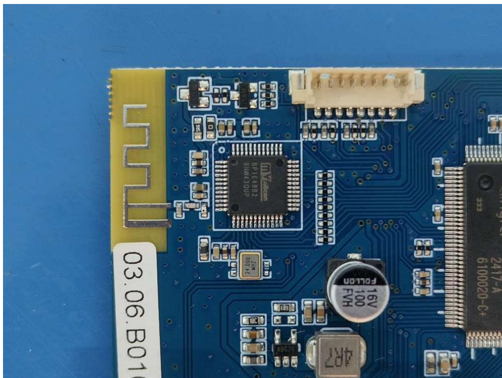
Internal view of Soundbar unit (Model:D51)
