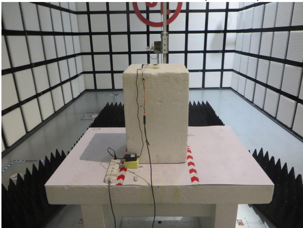
RADIATED RF MEASUREMENT SETUP (Above 1 GHz)
