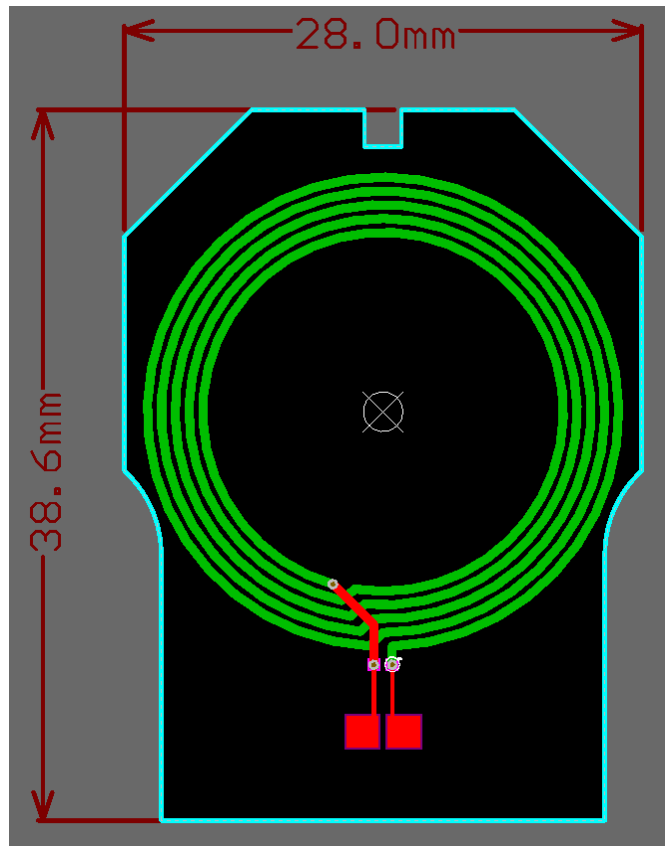
Pad detail
