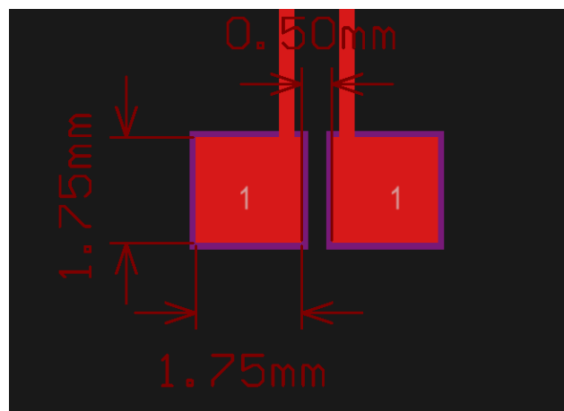
Pad detail
