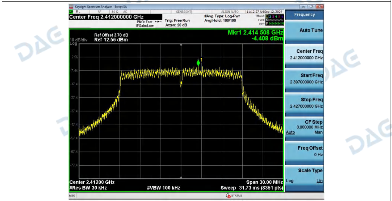
Power_Spectral_Density_NVNT_ANT1_802_11n(HT20)_2412
