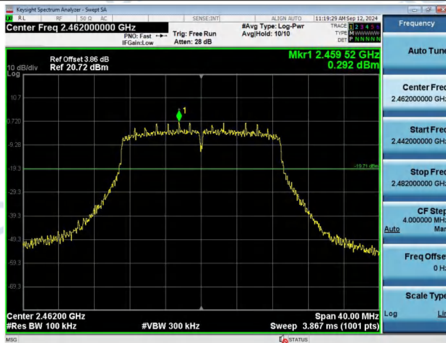
2_Spurious_Emission_NVNT_ANT1_802_11n(HT20)_2462
