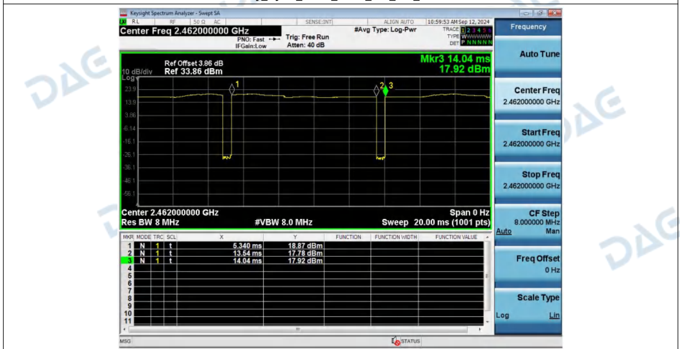
Duty_Cycle_NVNT_ANT1_802_11b_2462
