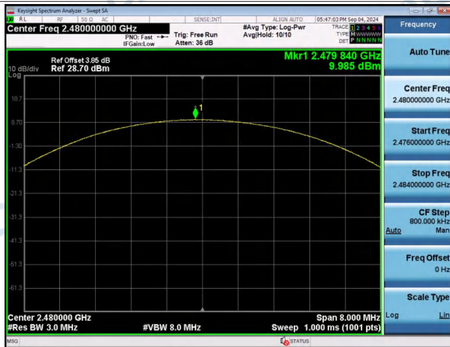
Peak_Output_Power_NVNT_ANT1_3-DH5_2480_00
