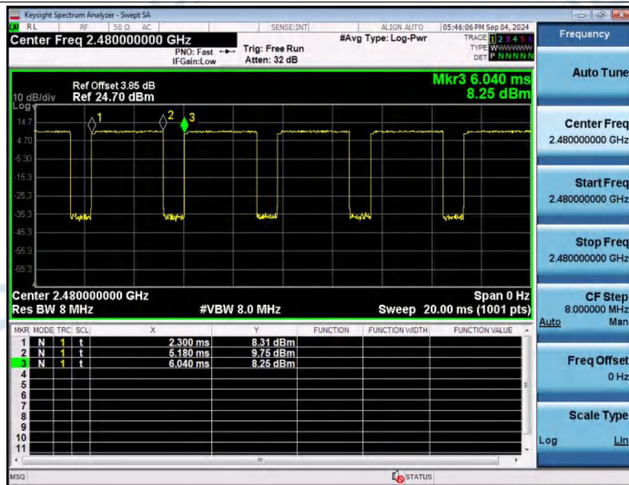
Duty_Cycle_NVNT_ANT1_3-DH5_2480
