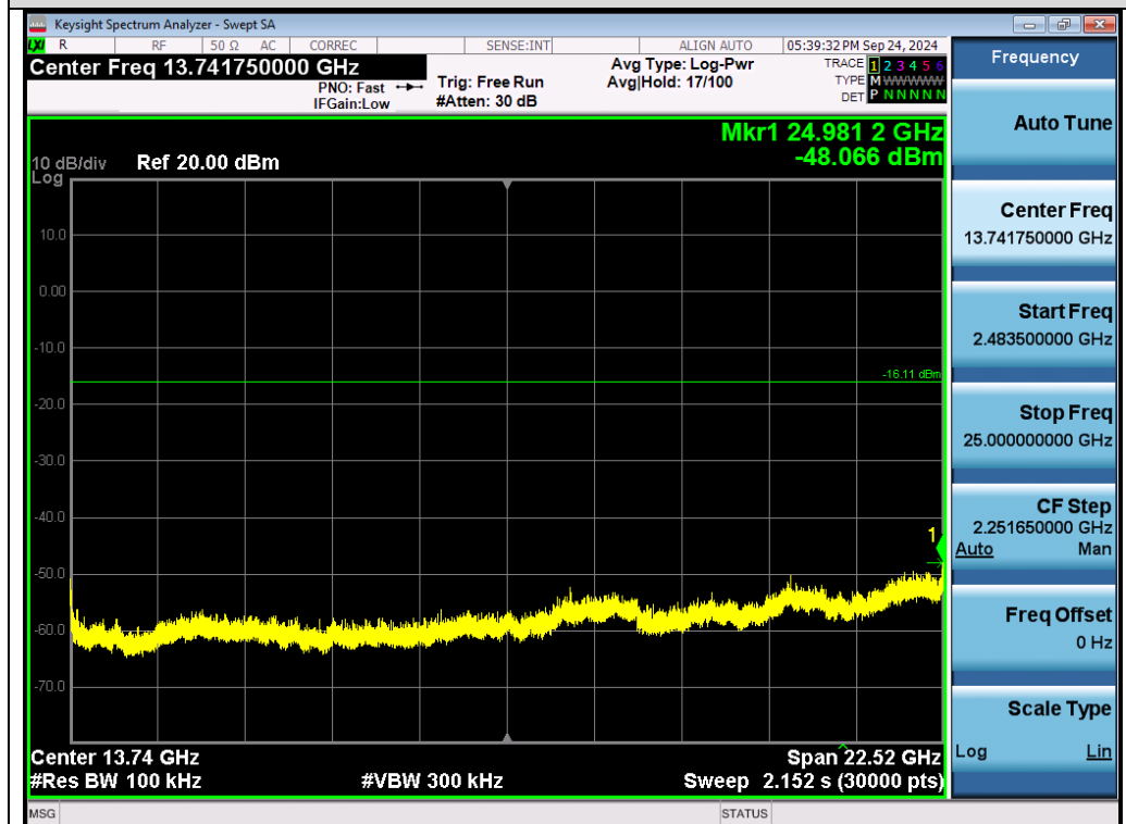
Test_Graph_Custom IEEE 802.11_Chain A_2445_MCS0_Higher Band Emissions
