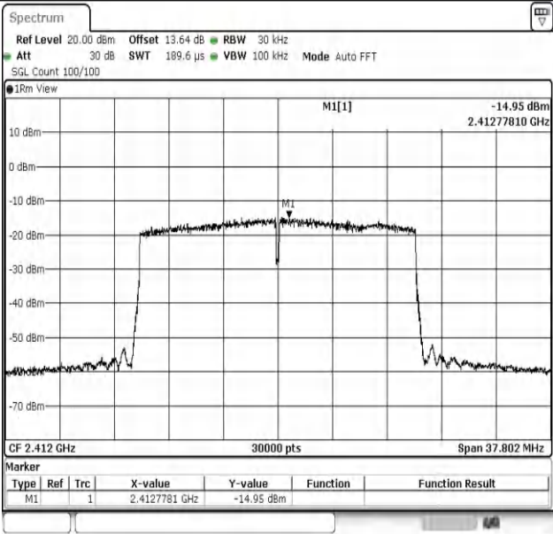
11AX20MIMO-Ant1-2412-PASS
