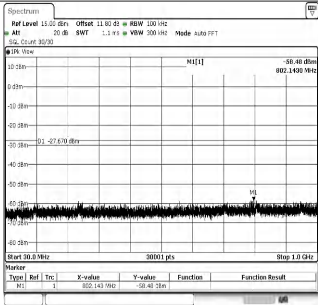
11G-Ant2-2412-30~1000-PASS
