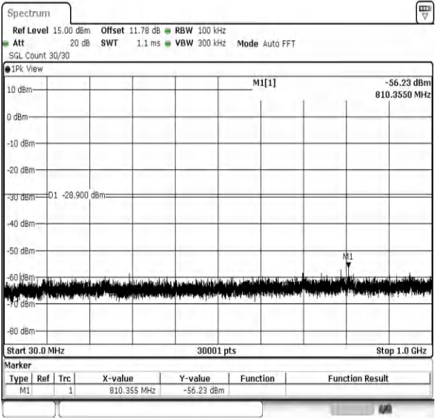
11B-Ant2-2437-30~1000-PASS
