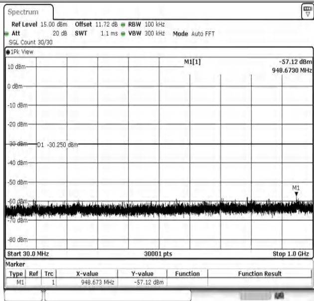
11B-Ant2-2462-30~1000-PASS
