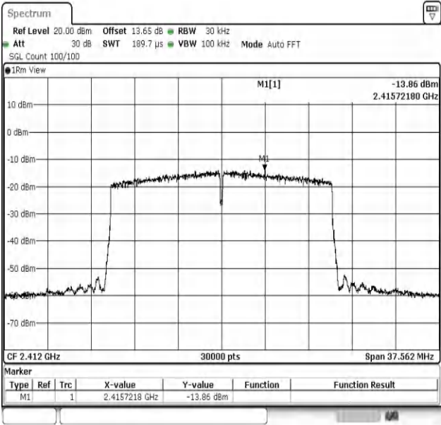
11AX20MIMO-Ant2-2412-PASS
