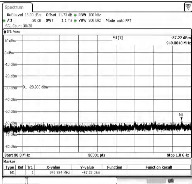
11B-Ant1-2462-30~1000-PASS
