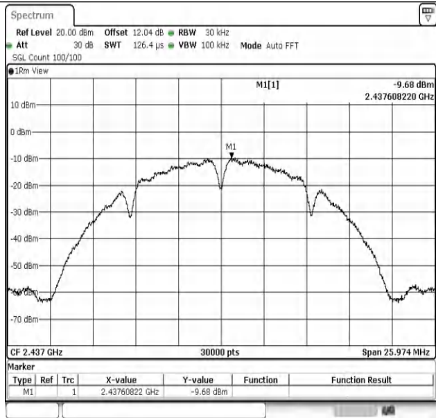
11B-Ant1-2437-PASS
