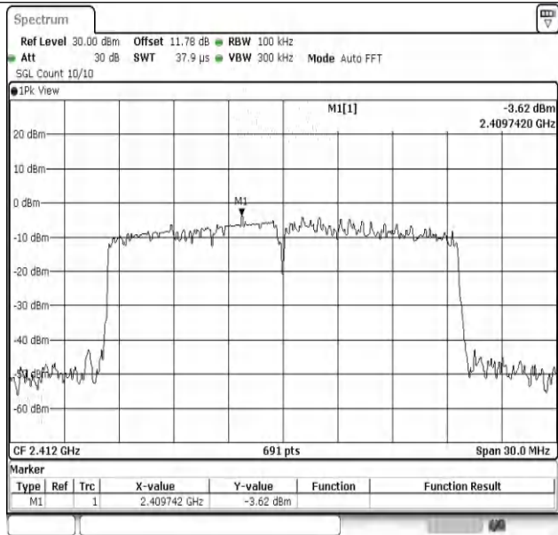
11AX20MIMO-Ant1-2412-0~Reference-PASS
