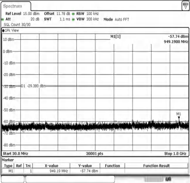
11B-Ant1-2437-30~1000-PASS
