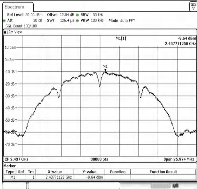
11B-Ant2-2437-PASS
