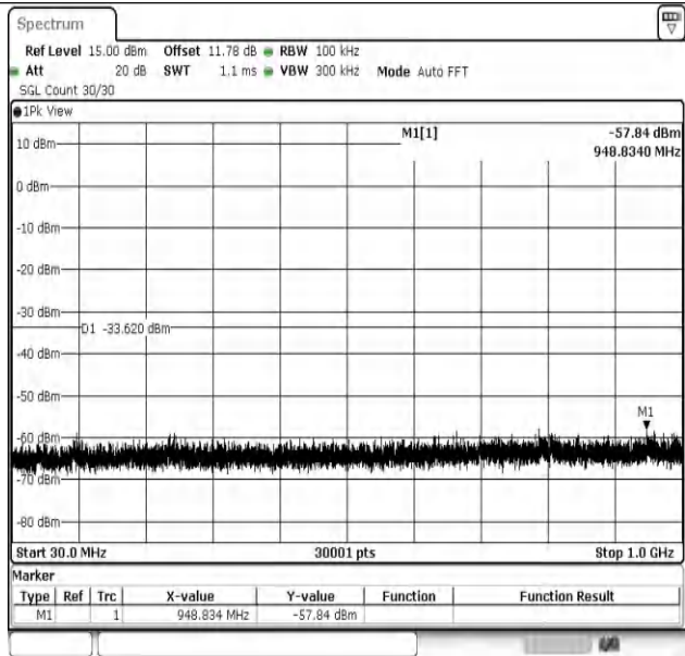
11AX20MIMO-Ant1-2412-30~1000-PASS
