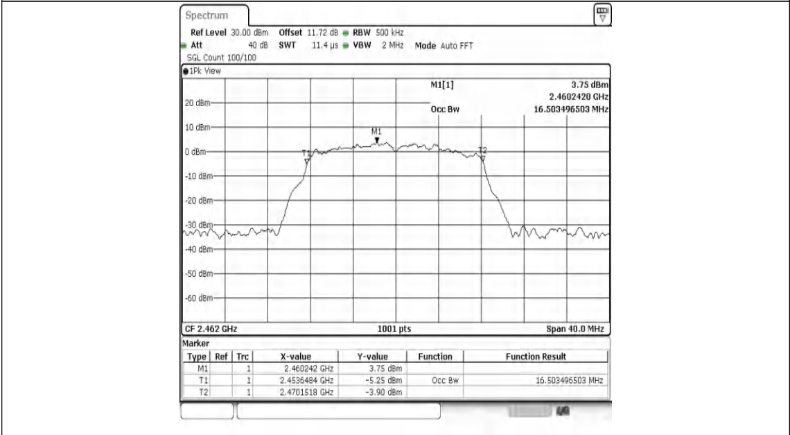
11G-Ant2-2462
