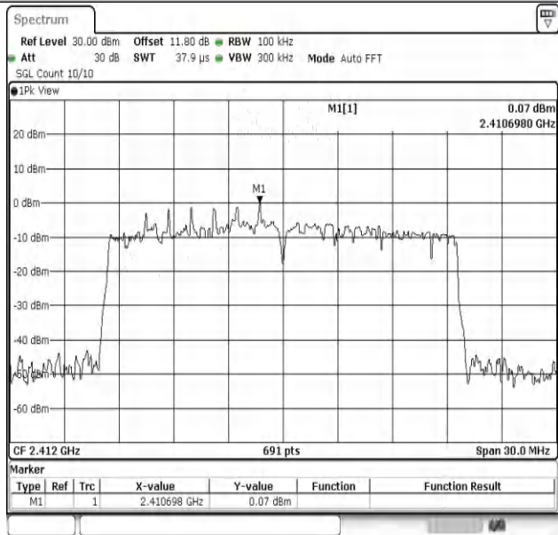
11AX20MIMO-Ant2-2412-0~Reference-PASS
