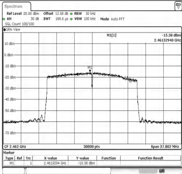
11AX20MIMO-Ant2-2462-PASS
