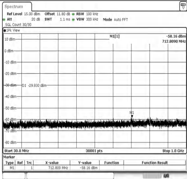
11AX20MIMO-Ant2-2412-30~1000-PASS
