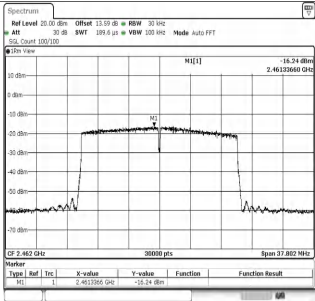
11AX20MIMO-Ant1-2462-PASS
