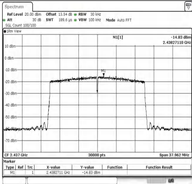
11AX20MIMO-Ant2-2437-PASS
