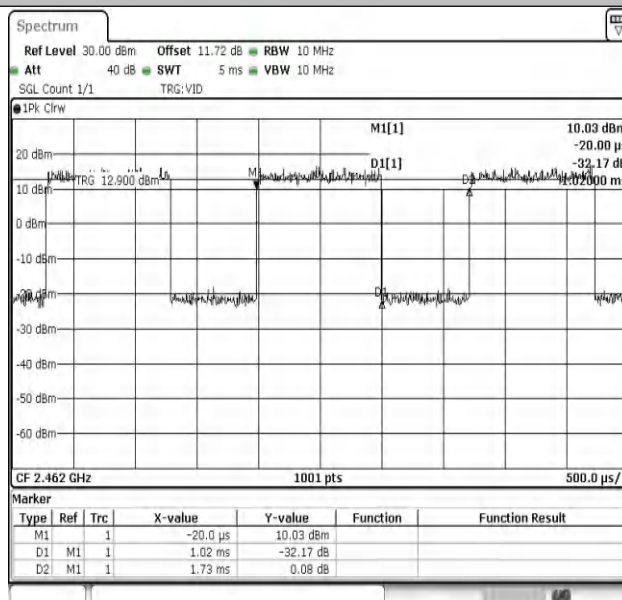
NTNV-11AX20MIMO-Ant2-2462
