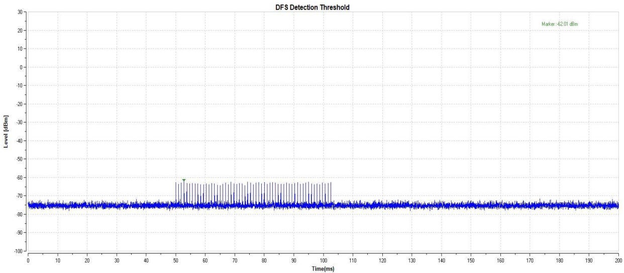
11AC20-5260-Type1-PASS
