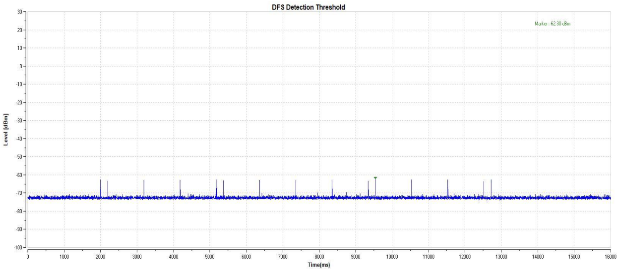
11AC20-5500-Type5-PASS
