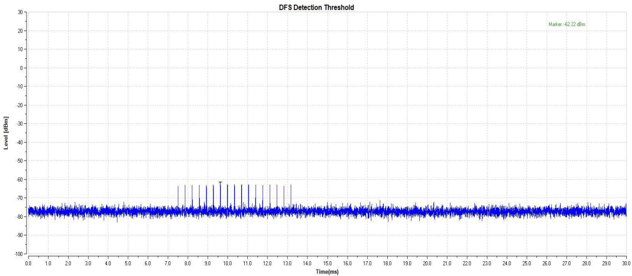
11AC40-5510-Type3-PASS
