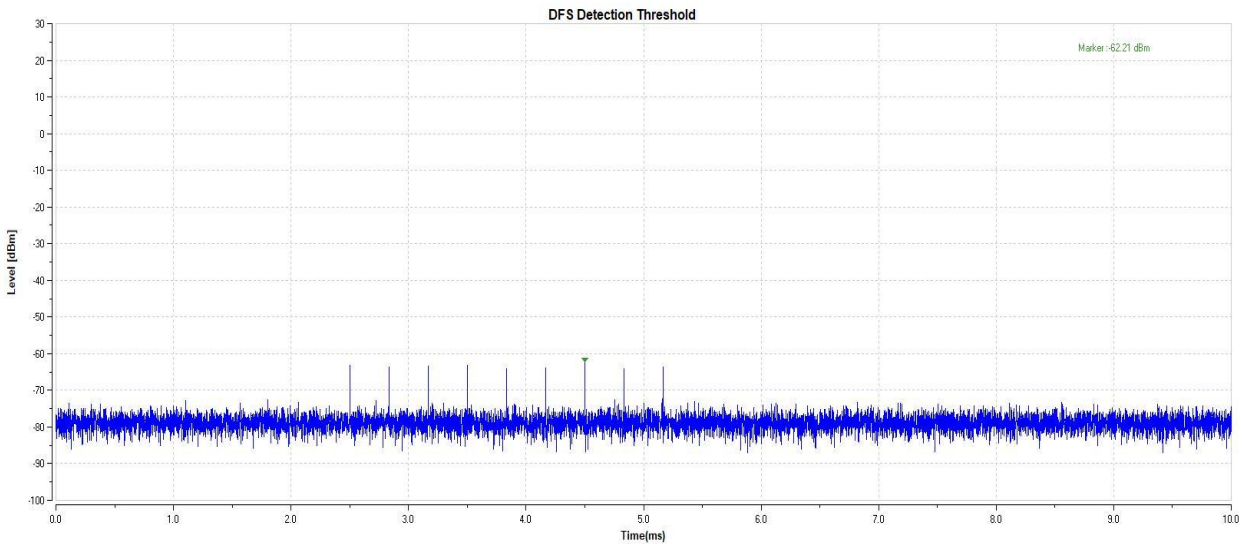
11AC40-5510-Type6-PASS
