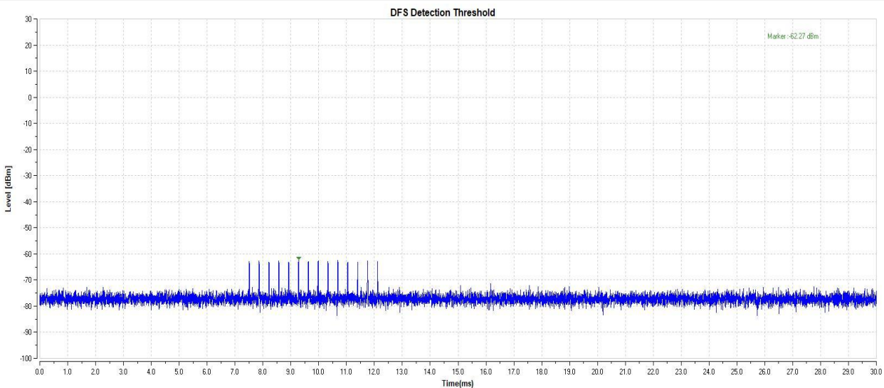
11AC20-5500-Type4-PASS
