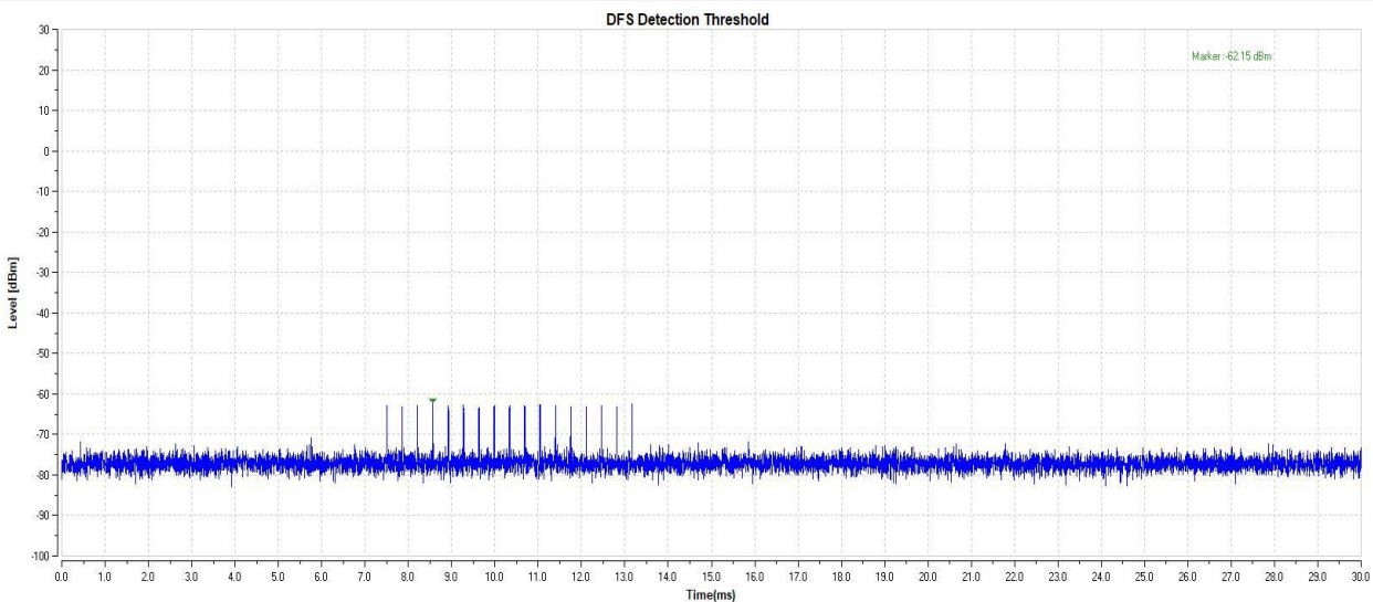
11AC80-5530-Type3-PASS
