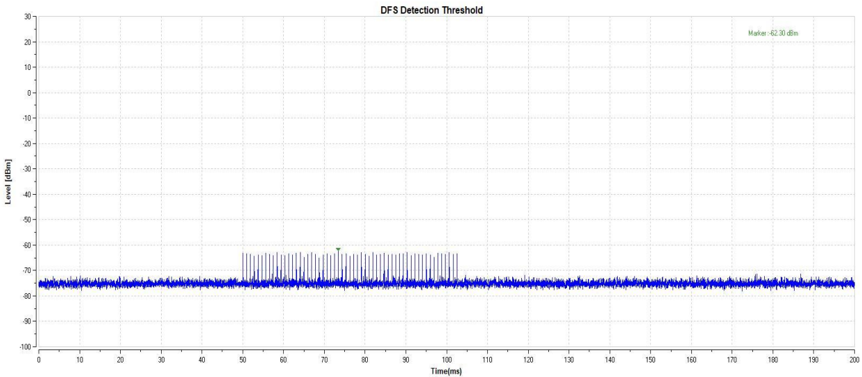
11AC80-5530-Type1-PASS
