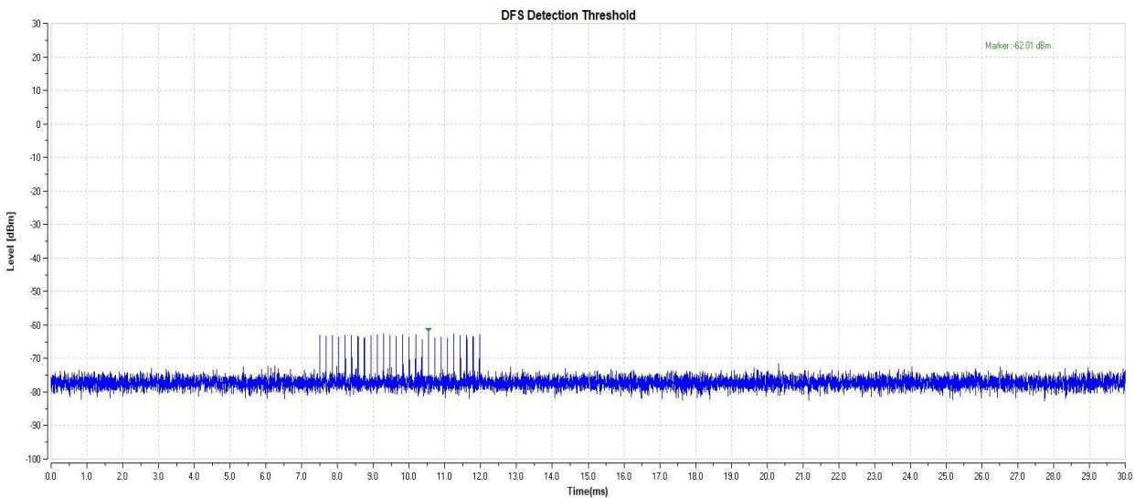
11AC20-5260-Type2-PASS
