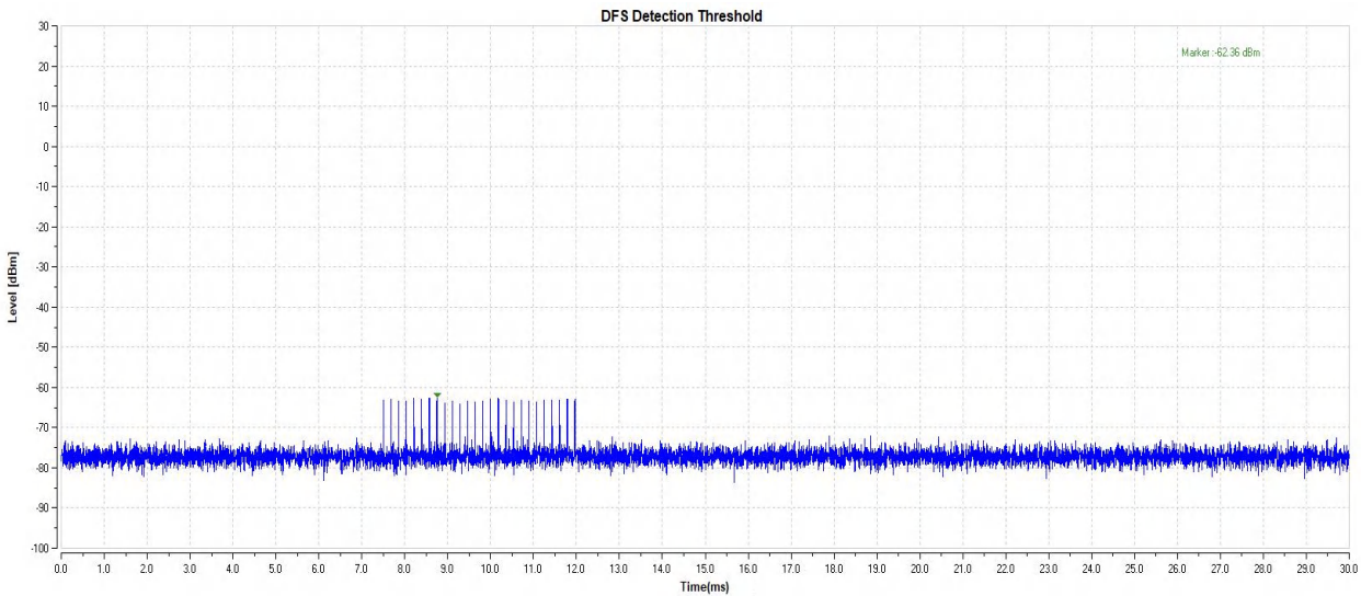
11AC20-5500-Type2-PASS
