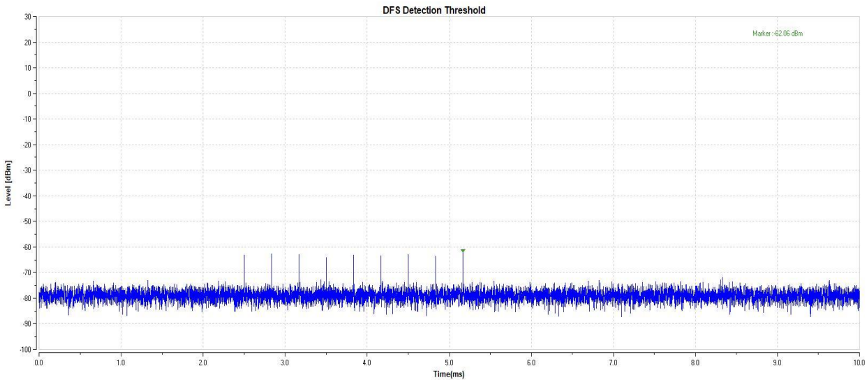
11AC20-5260-Type6-PASS
