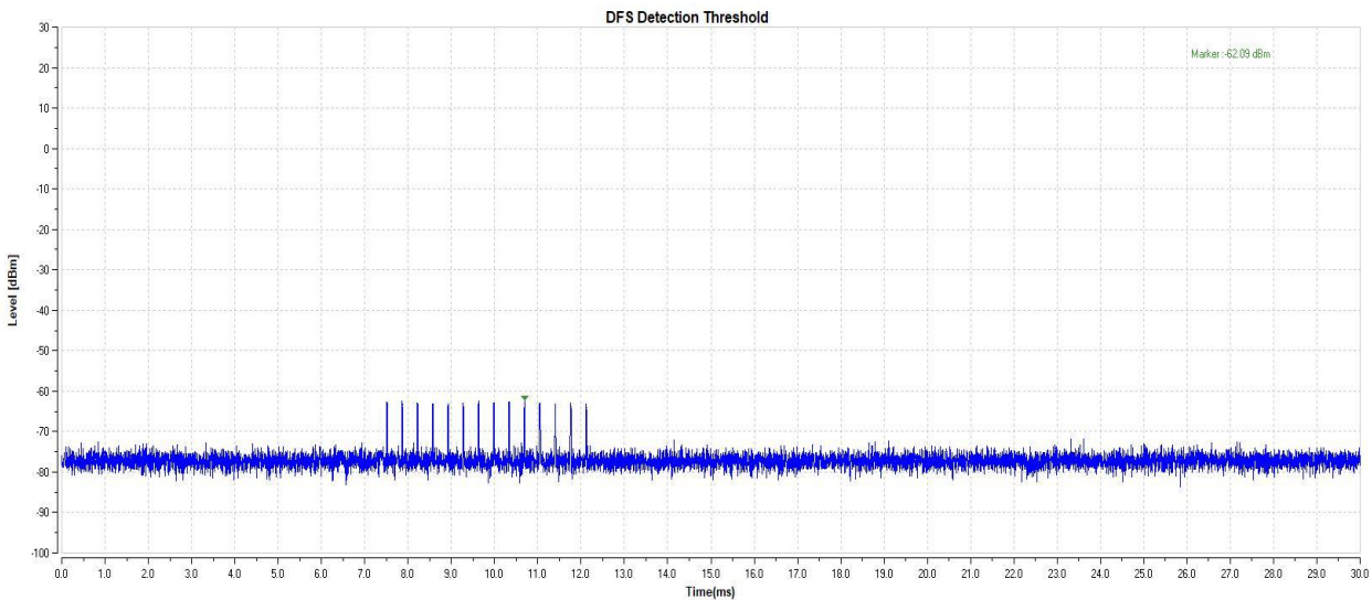
11AC20-5260-Type4-PASS
