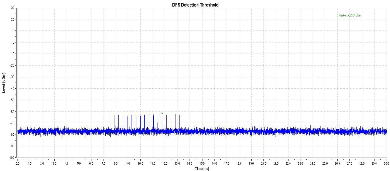
11AC20-5500-Type3-PASS
