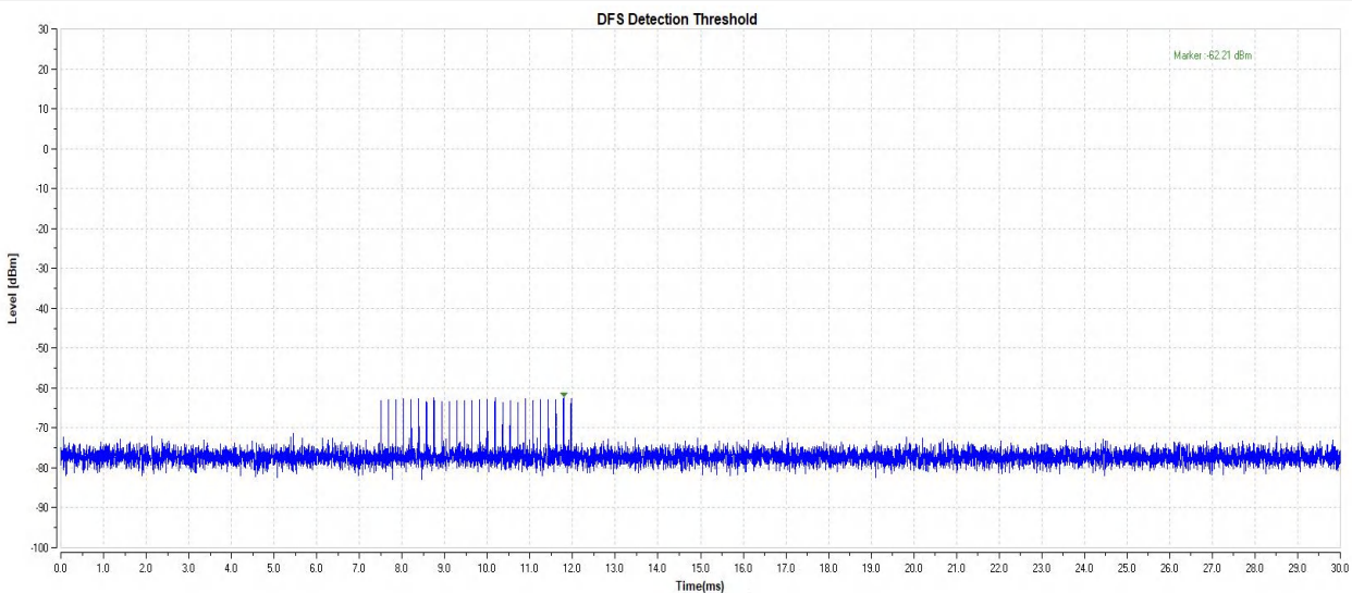
11AC40-5510-Type2-PASS
