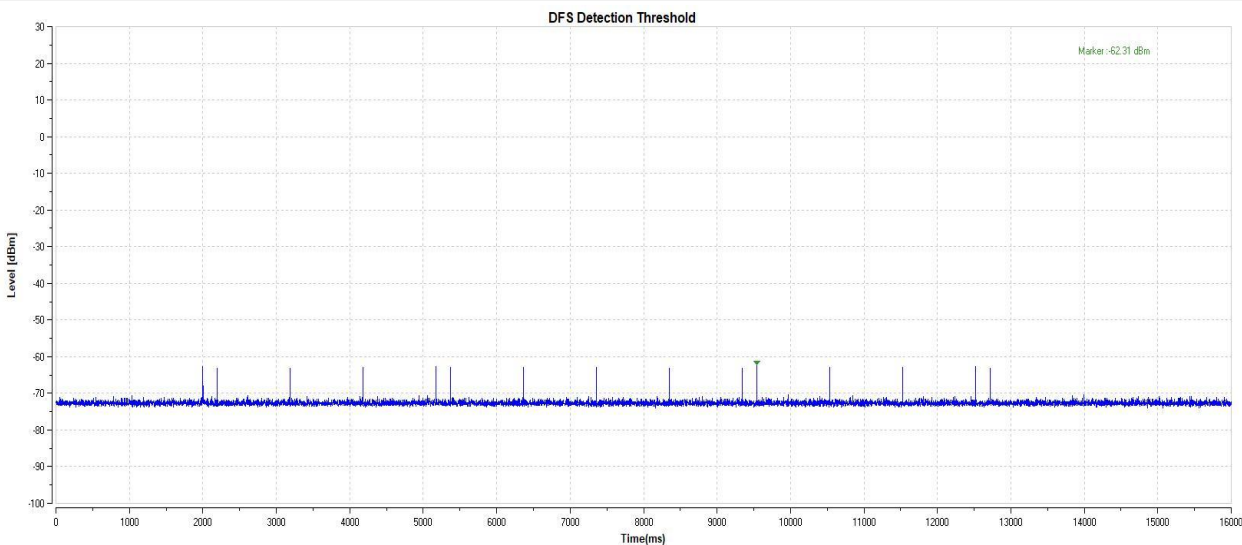
11AC20-5260-Type5-PASS
