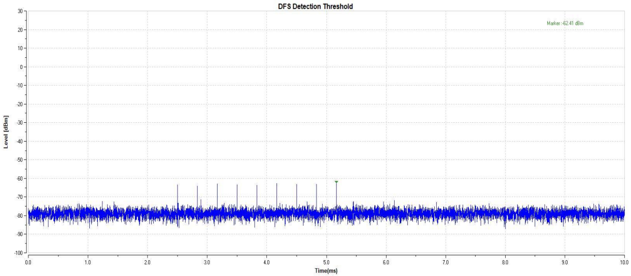
11AC20-5500-Type6-PASS
