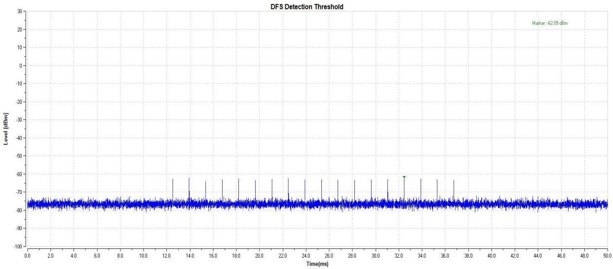
11AC20-5260-Type0-PASS
