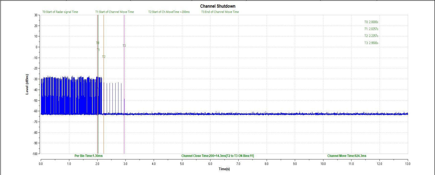
11AC80_5290
