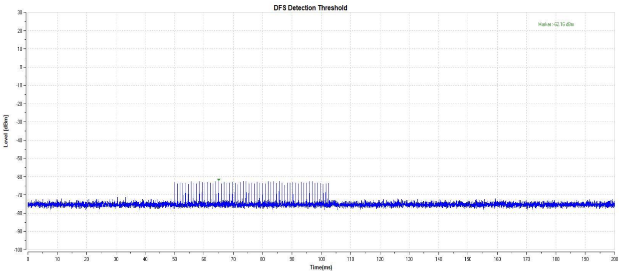
11AC40-5510-Type1-PASS
