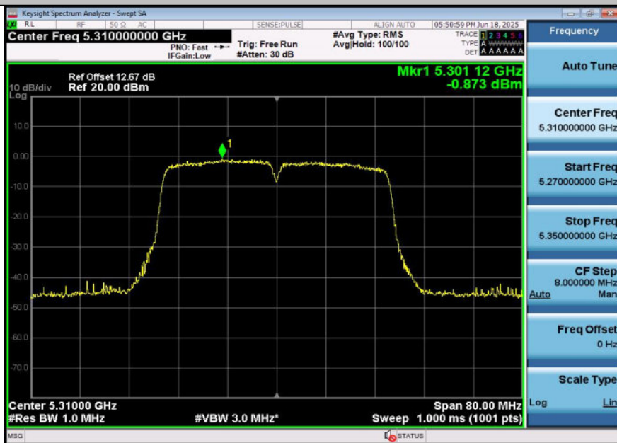
11N40SISO-Ant1-5310-PASS
