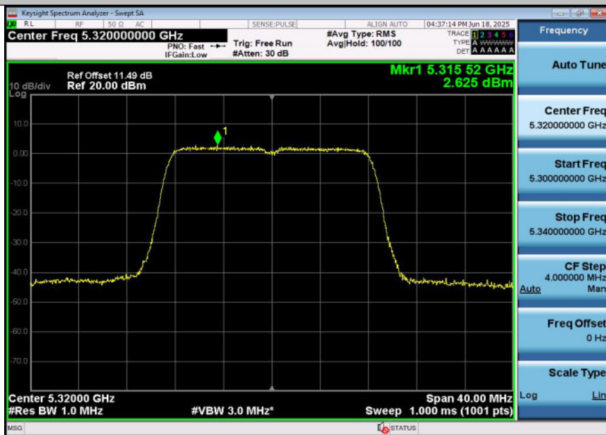
11A-Ant1-5320-PASS
