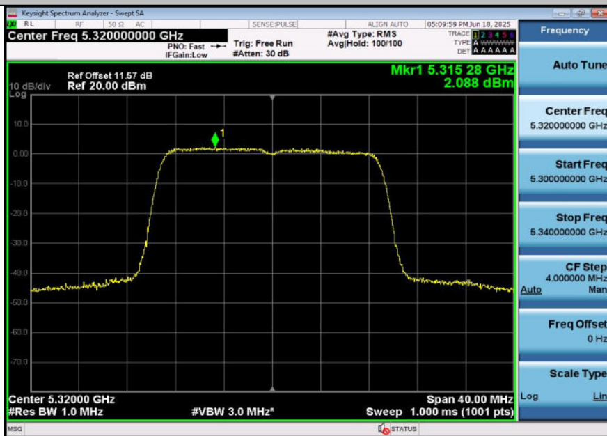
11N20SISO-Ant1-5320-PASS
