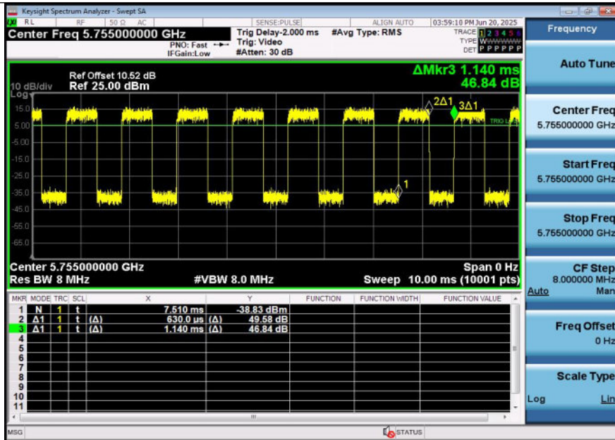
NTNV-11AX40SISO-Ant2-5755
