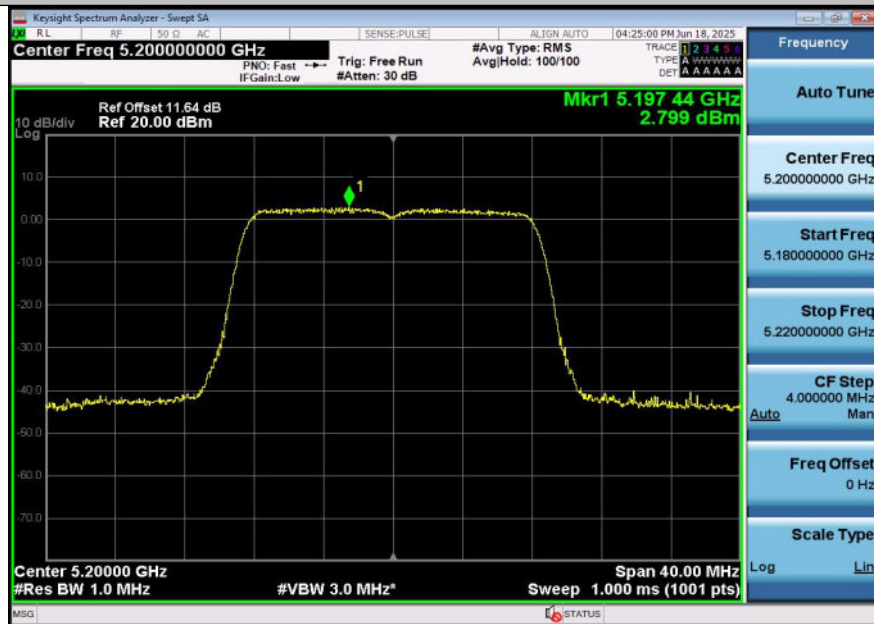
11A-Ant1-5200-PASS
