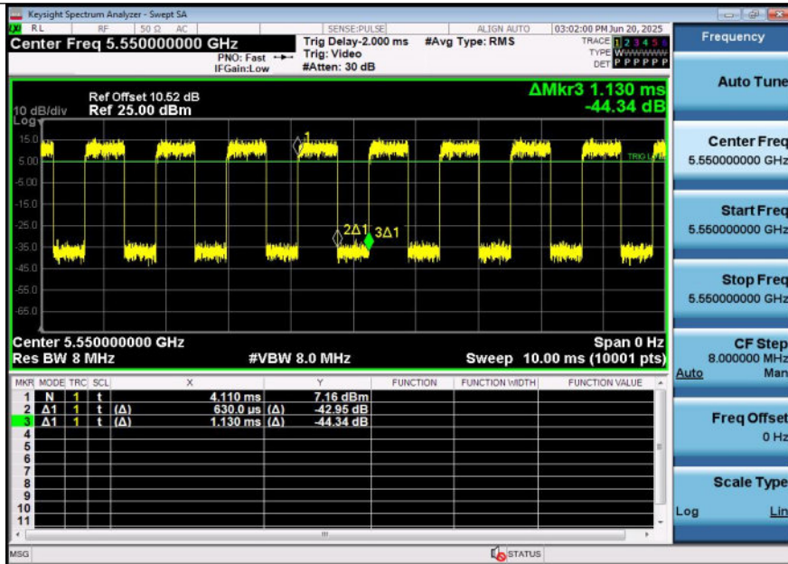
NTNV-11AC40SISO-Ant2-5550
