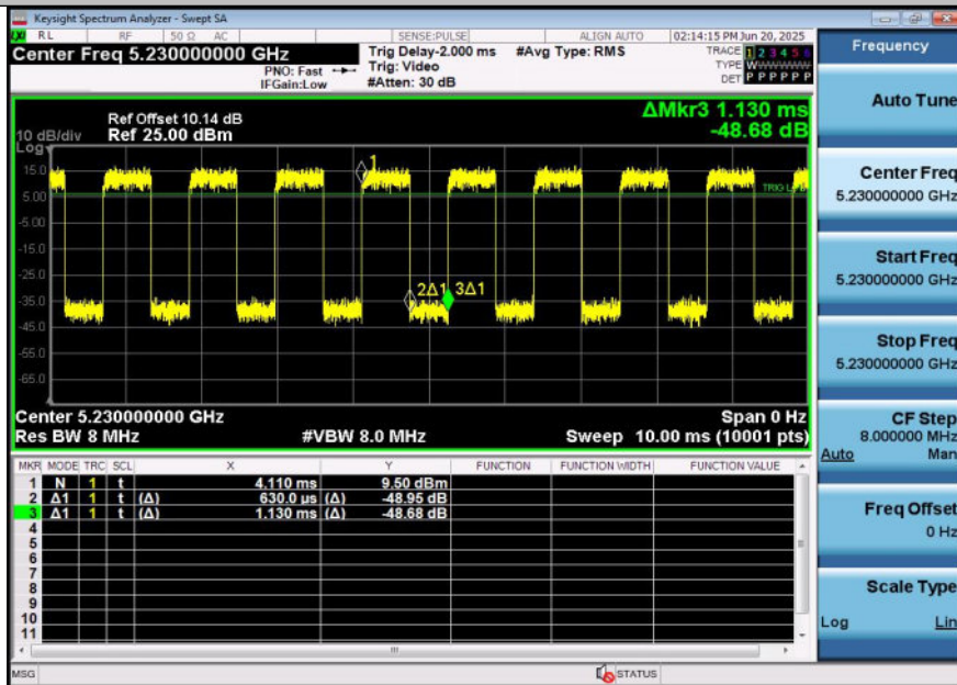
NTNV-11N40SISO-Ant2-5230
