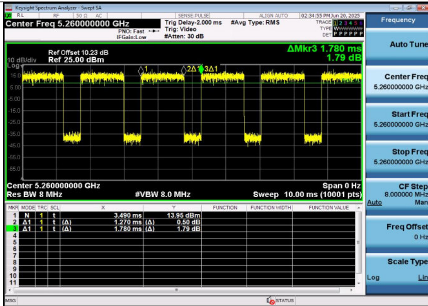
NTNV-11AC20SISO-Ant2-5260
