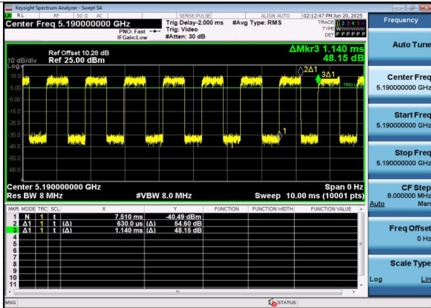
NTNV-11N40SISO-Ant2-5190
