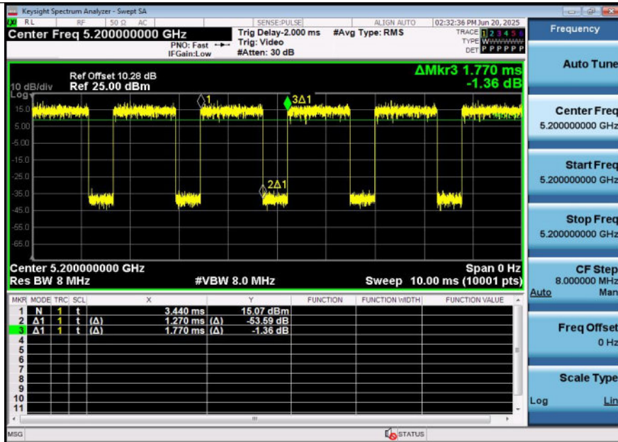
NTNV-11AC20SISO-Ant2-5200
