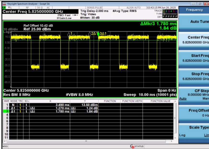
NTNV-11AX20SISO-Ant2-5825
