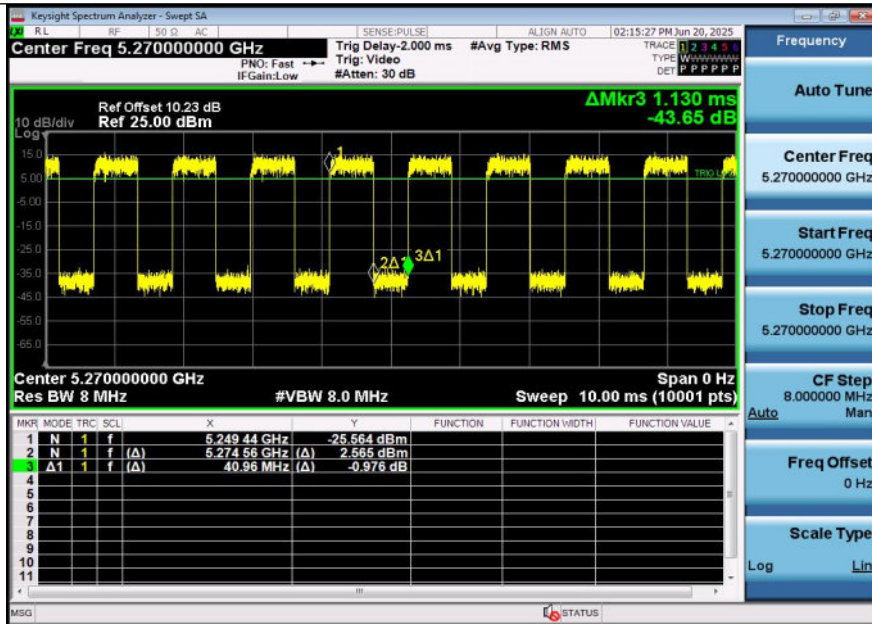
NTNV-11N40SISO-Ant2-5270
