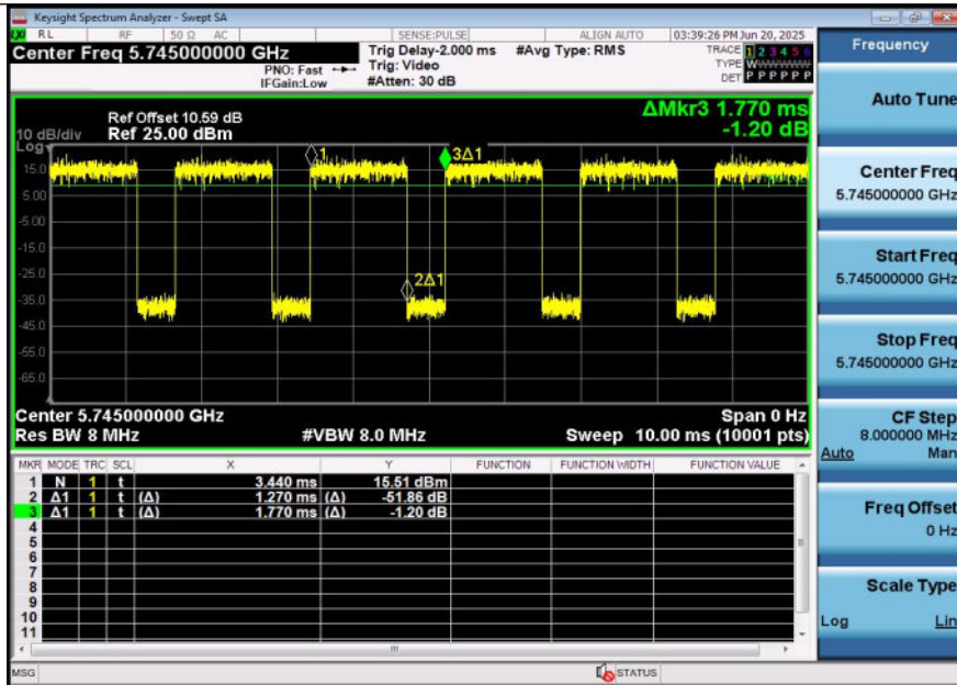
NTNV-11AX20SISO-Ant2-5745
