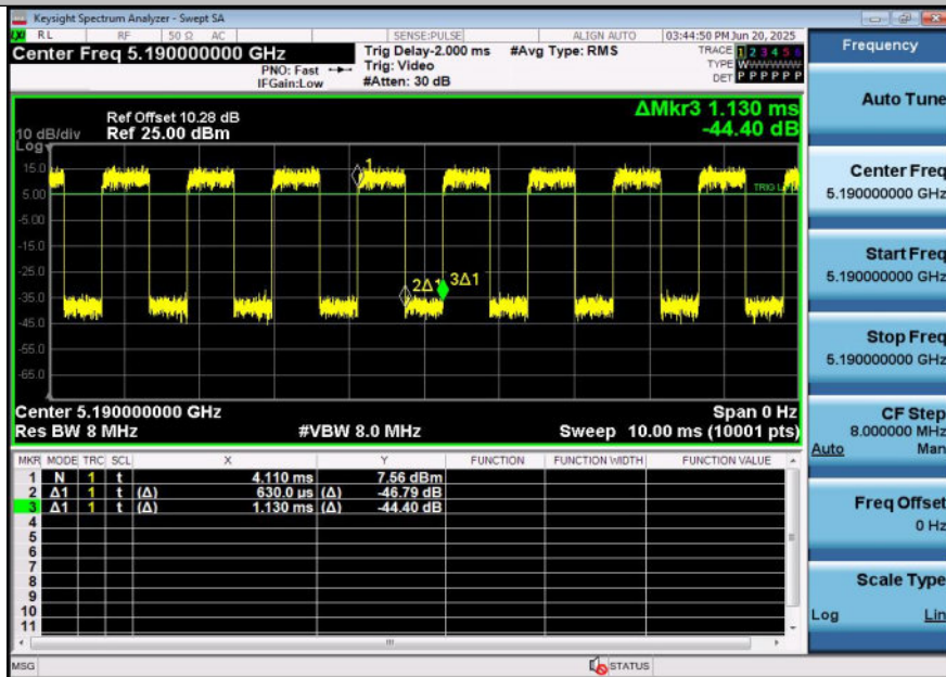
NTNV-11AX40SISO-Ant2-5190
