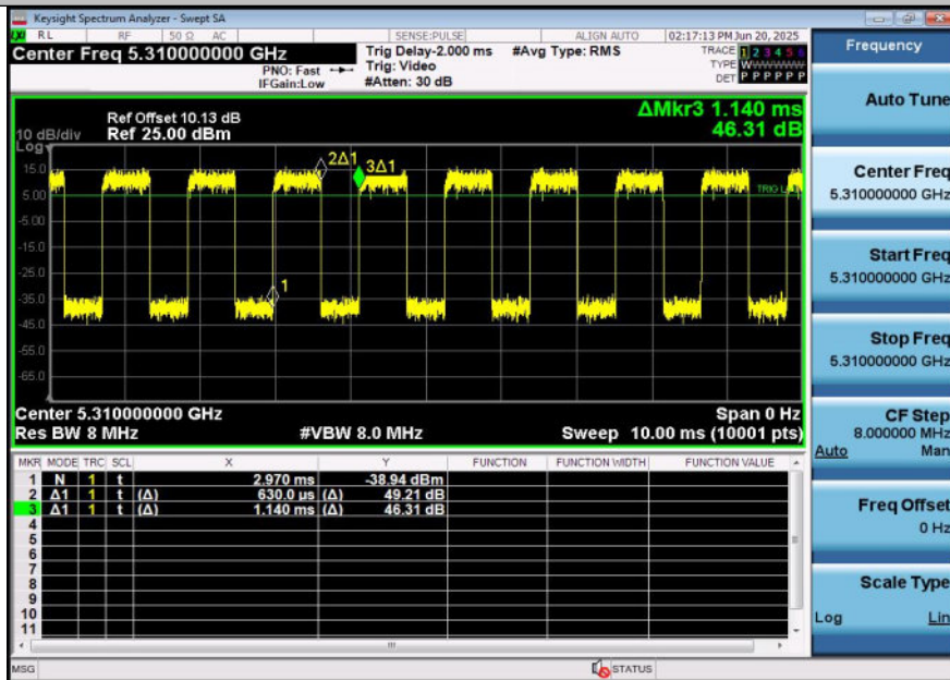
NTNV-11N40SISO-Ant2-5310
