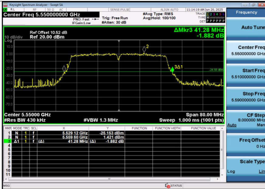
11AX40SISO-Ant1-5550
