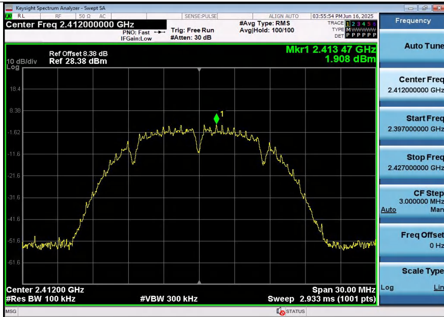
11B-Ant2-2412-0~Reference-PASS
