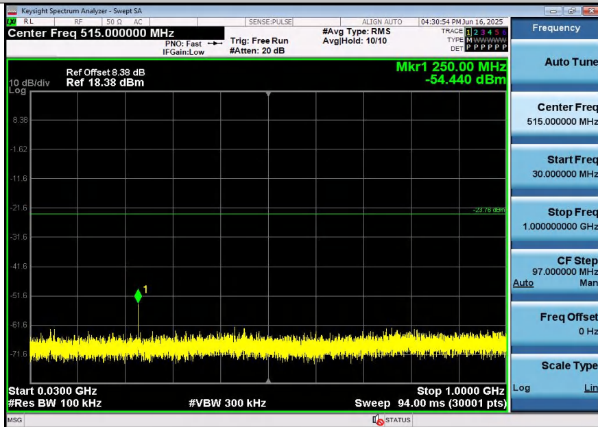
11G-Ant2-2437-30~1000-PASS
