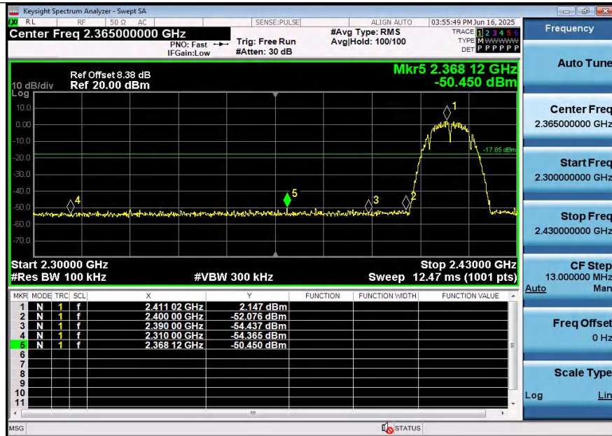
11B-Ant2-2412-PASS
