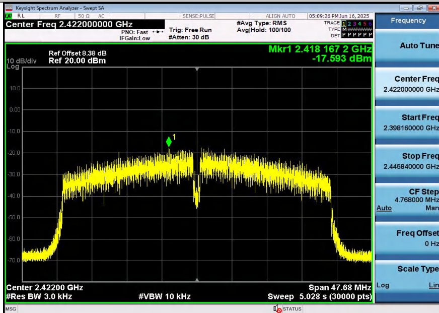
11N40SISO-Ant2-2422-PASS
