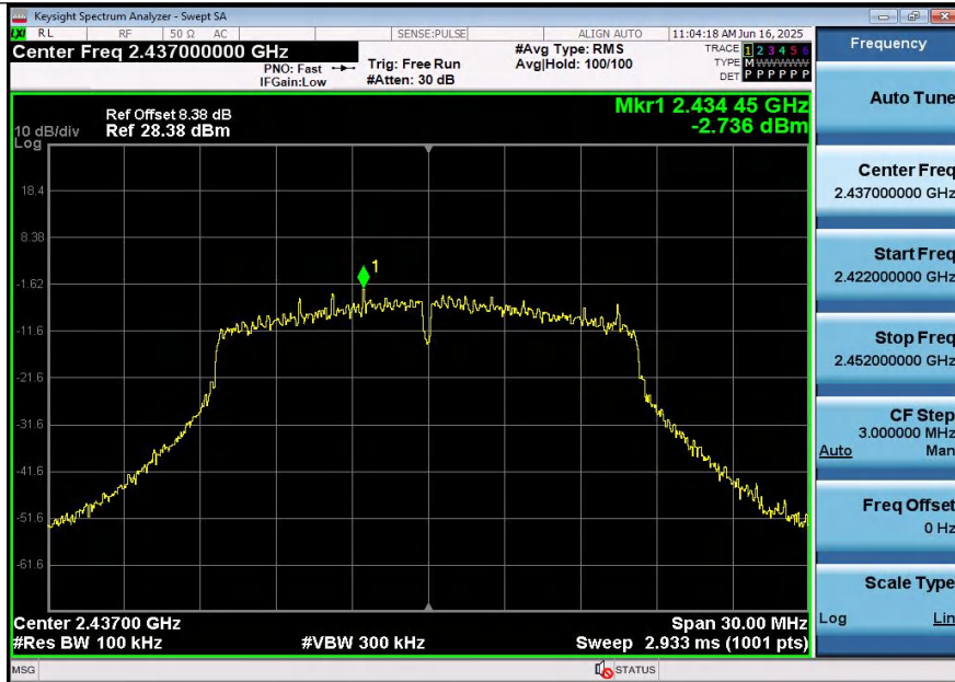
11G-Ant1-2437-0~Reference-PASS
