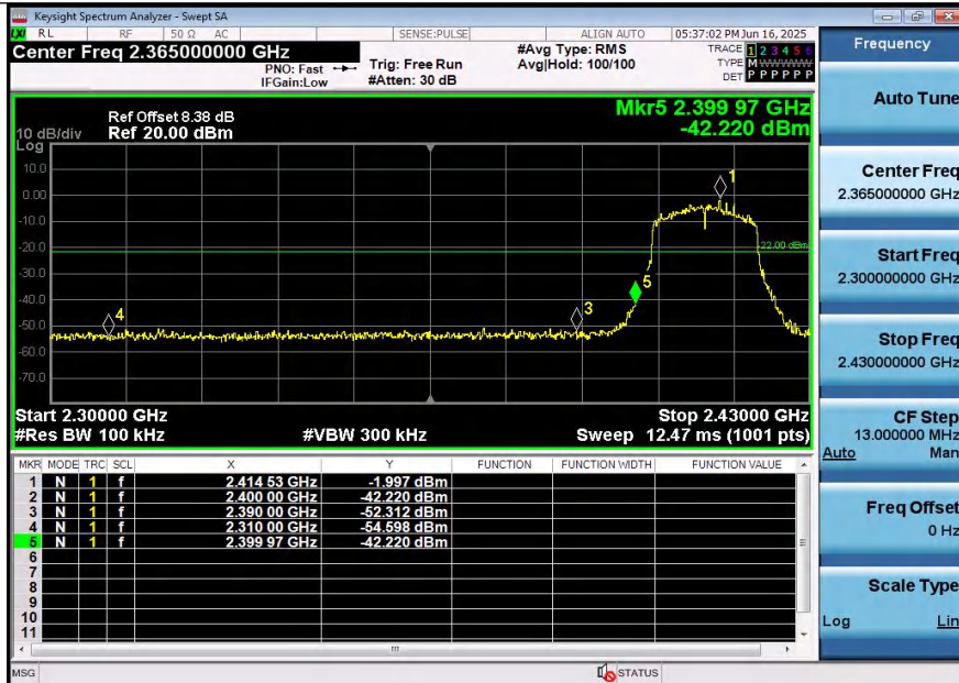
11AX20SISO-Ant2-2412-PASS
