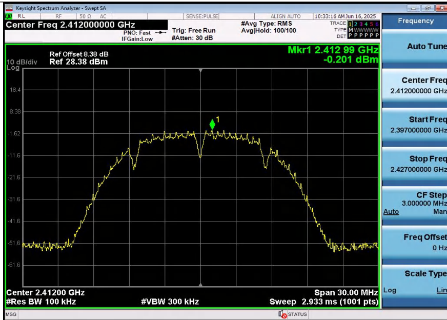
11B-Ant1-2412-0~Reference-PASS
