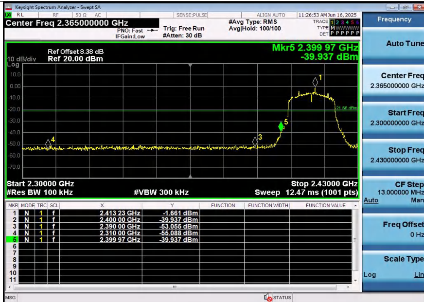
11N20SISO-Ant1-2412-PASS
