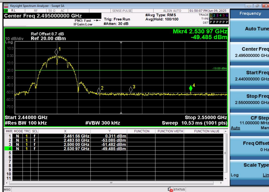
11B-Ant1-2462-PASS
