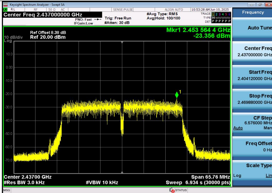
11N40SISO-Ant2-2437-PASS
