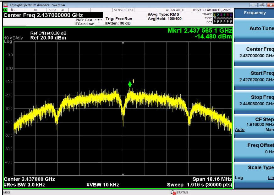
11B-Ant2-2437-PASS
