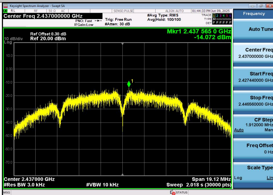
11B-Ant1-2437-PASS
