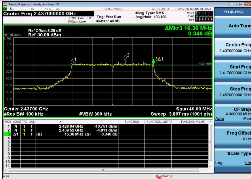
11G-Ant2-2437-PASS
