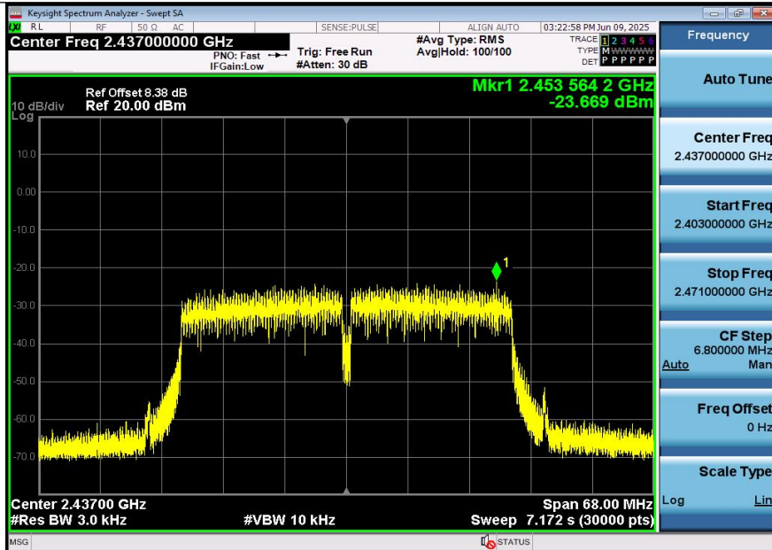
11N40SISO-Ant1-2437-PASS
