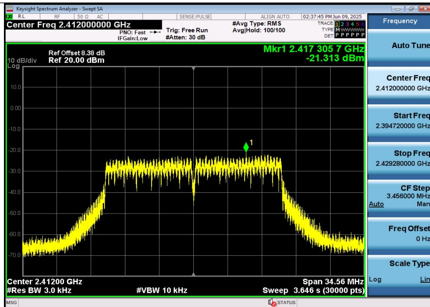
11N20SISO-Ant1-2412-PASS
