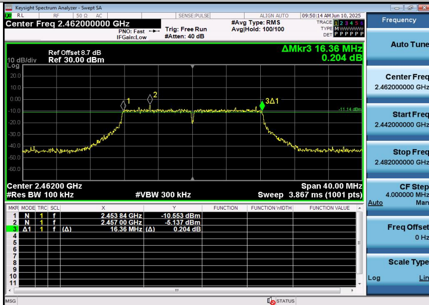
11G-Ant2-2462-PASS
