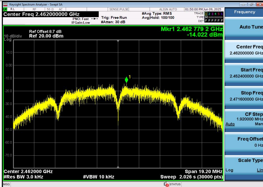
11B-Ant1-2462-PASS
