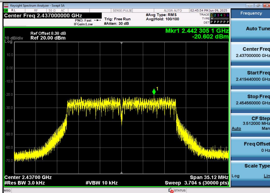
11N20SISO-Ant1-2437-PASS
