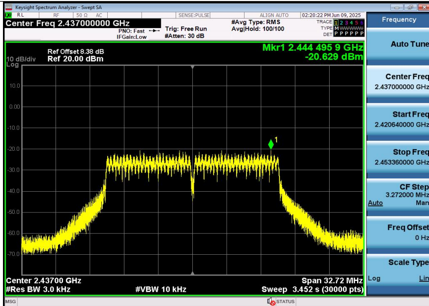
11G-Ant1-2437-PASS
