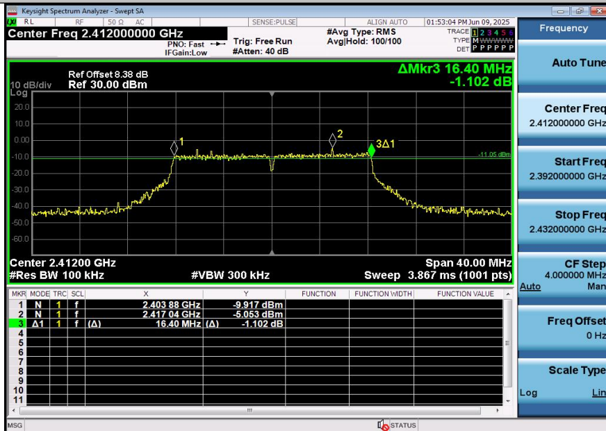
11G-Ant1-2412-PASS
