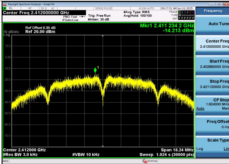
11B-Ant2-2412-PASS
