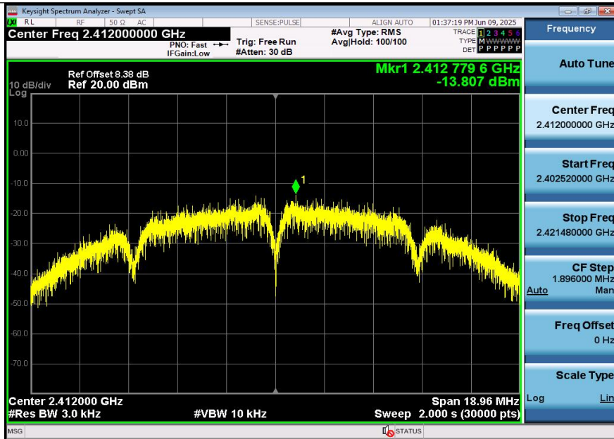
11B-Ant1-2412-PASS
