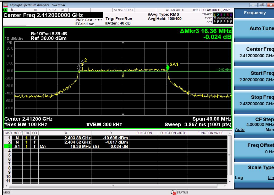
11G-Ant2-2412-PASS
