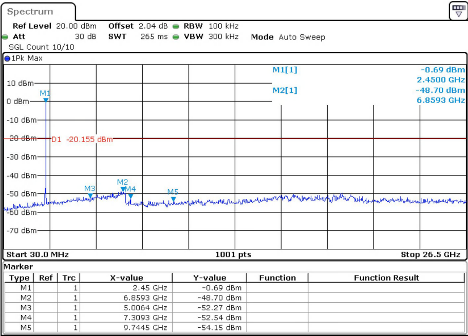
Tx. Spurious BLE 1M 2440MHz Emission
