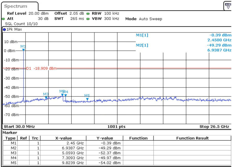
Tx. Spurious BLE 1M 2480MHz Emission
