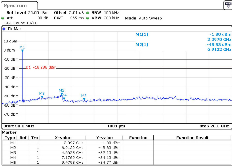
Tx. Spurious BLE 1M 2402MHz Emission
