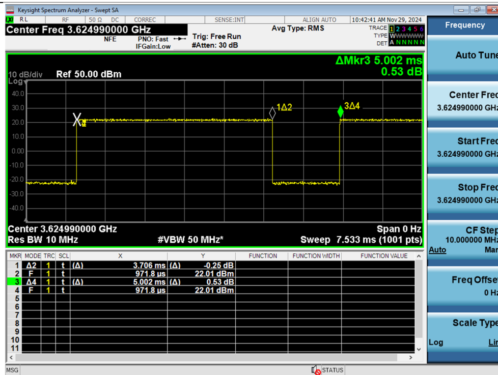
Measurement Result of SJ-ORU4402-N48US Transmit On/Off Timing
